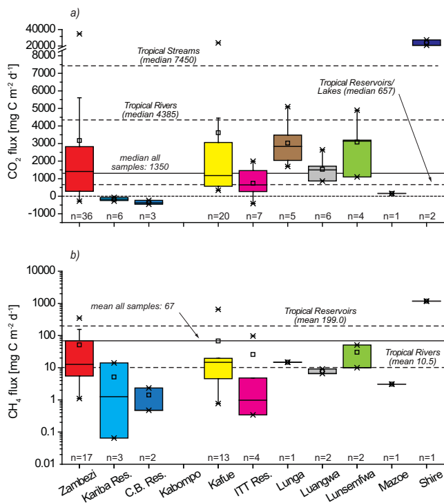
Figure 9. Measured range in (a) CO 2 fluxes and (b) CH 4 fluxes (note the log scale in the latter) for the Zambezi mainstem, tributaries and reservoirs. Box plots show the range, percentile, median, mean and outliers. Dashed lines in (a) represent global median CO 2 efflux for tropical rivers, streams and lakes/reservoirs based on Aufdenkampe et al. (2011), while in (b) they represent the global mean CH 4 emission for tropical rivers and reservoirs as suggested by Bastviken et al. (2011). Solid lines represent median CO 2 emissions (a) and mean CH 4 flux (b) of all sites and over the entire sampling period.
