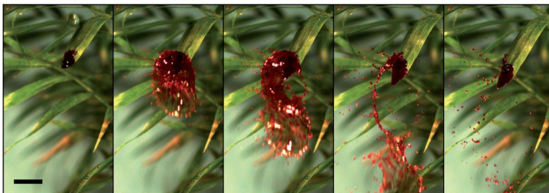
Fig. 4 Splash by raindrop (diameter 5.0 mm, speed 7 m/s) and fragmentation of a contaminated sessile drop on an Areca Palm leaf. We = 3500 and K = 45,000 . The first snapshot is taken at 2 milliseconds prior to the raindrop's impact. Subsequent snapshots at 2, 4, 7, and 11 ms after impact are then displayed. The largest ejected droplet is 1.6 mm in diameter. Scale bar is 1 cm.
