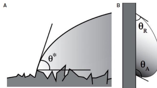
Fig. 2 (A) Apparent contact angle \theta^* of a drop on a rough horizontal surface, such as a leaf. (B) The apparent contact angle of a drop on a vertical surface resides between the advancing contact angle \theta_A and the receding contact angle \theta_R : \theta_R \leq \theta^* \leq \theta_A . The difference between the advancing and receding contact angles allow for a drop to resist gravitational pull. It can thus stick to surfaces such as leaves (Bourouiba and Bush 2013).
