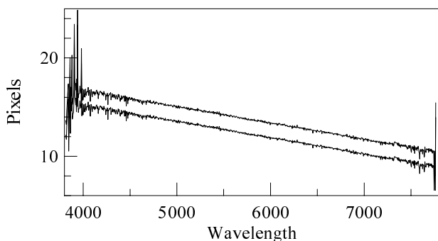
Fig. 4. An example of the spectra positions after the first processing (model #1, spectra separation of 1.5 pxl). In spite of noise, a reliable estimate of the spectra positions is easily obtained.
