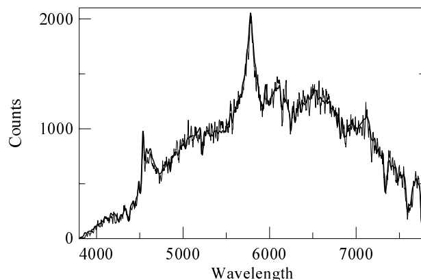
Fig. 5. Model #1: original (thick line) and extracted (thin line) spectra of the bright component A for a separation of 0.5 pxl between A and B_1 .
