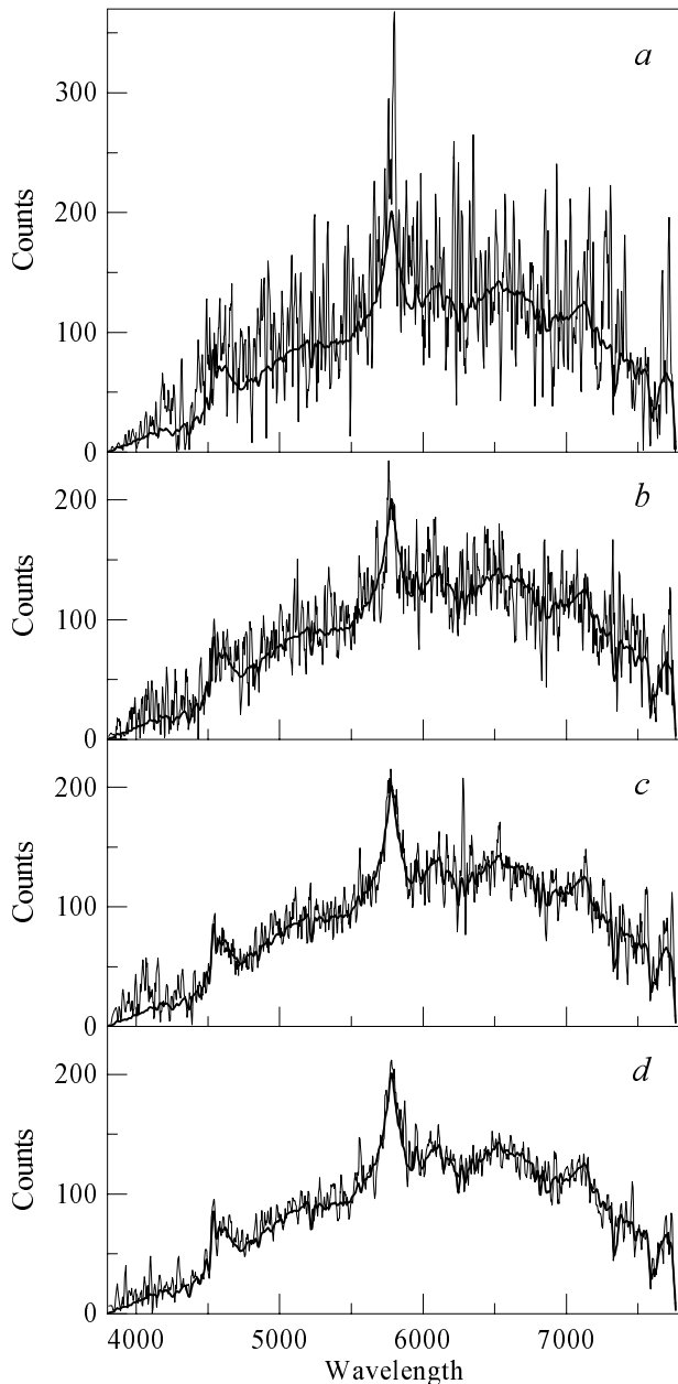
Fig. 7. Model #2: extracted spectra of the faint component B_2 (thin lines) for several separations between A and B_2 : a) 0.5 psl, b) 1.5 psl, c) 2.5 psl, d) 3.5 psl. The original spectrum is displayed with a thick line.
