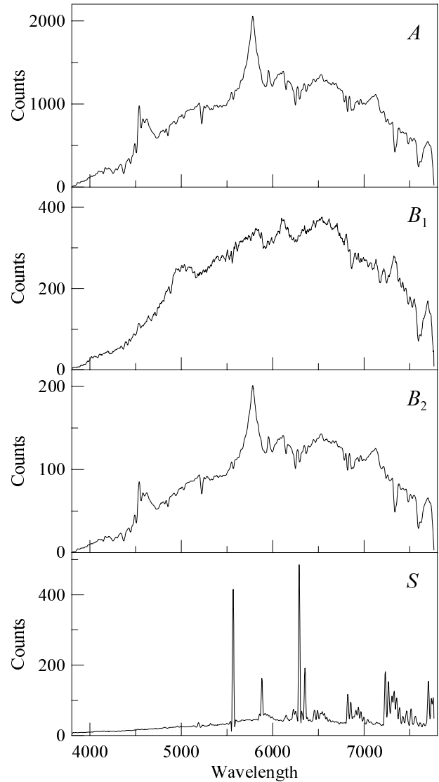
Fig. 2. Spectra that have been used for the CCD data simulations. From top to bottom: bright component ( A ), faint component (versions B_1 and B_2 ), night sky ( S ). See text for details.
