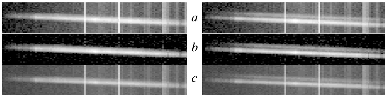
Fig. 3. Two examples of simulated spectral data in the case of model #1. As in Fig. 1, the size of each single image is 990 \times 26 pxl, and the direction of dispersion is horizontal. Separations between the spectra along the vertical (spatial) direction are 2 pxl (left panel) and 4 pxl (right panel). From top to bottom: a ) simulated spectral data, b ) spectral data after sky subtraction, c ) associated standard deviations.
