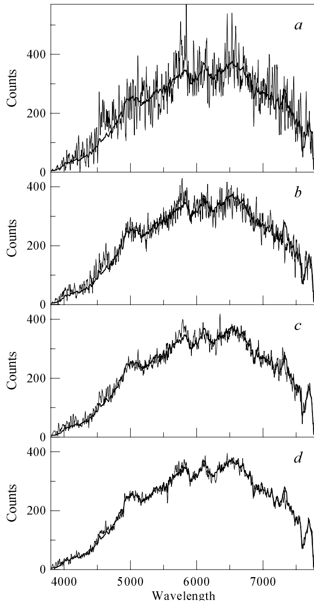
Fig. 6. Model #1: extracted spectra of the faint component B_1 (thin lines) for several separations between A and B_1 : a) 0.5 pxl, b) 1.5 pxl, c) 2.5 pxl, d) 3.5 pxl. For comparison, the thick lines represent the original spectrum.
