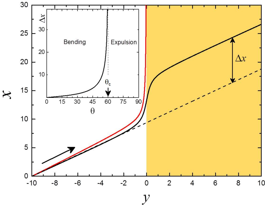
Figure 5. Trajectory x(y) of a magnet launched from x_0 = 0 , y_0 = -10 towards a conducting plane for b = 1 , z_0 = 1 and (red) a = 1 ; (black) a = 1.1 . The deflection is bigger as a decreases towards the critical value a = b/z_0^2 = 1 . For smaller values of a , the magnet is completely repelled by the conductor. Inset: \Delta x as a function of the initial angle \theta for C = 0.5 , F = 1 and z_0 = 1 . The critical angle \theta_c above which the magnet does not penetrate in the region covered by the conducting layer is indicated. Bending (exclusion) of the vortex trajectory corresponds to the black (red) line in the main panel. The x and y coordinates are normalized by z_0 .
