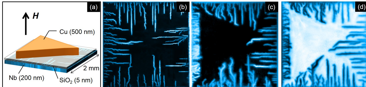
Figure 1. (a) Sketch of the sample layout. Panels (b) and (c) show magneto-optical images taken at T = 2.5 K after zero-field cooling in H = 10 Oe for the Nb sample before (b) and after (c) covering it with the Cu triangle. The bright areas correspond to the highest magnitudes of the magnetic field, while the dark areas represent the lowest fields. Panel (d) shows a MOI picture of the Nb sample with the Cu triangle after field-cooling in H = 10 Oe down to T = 2.5 K and subsequently turning off the magnetic field.
