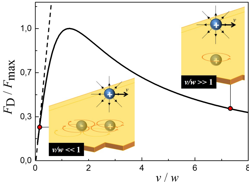
Figure 3. Comparison of the models developed by Baker-Rojo [11] (dotted line) and that of Reitz [25] (solid line) for the drag force acting on a moving monopole in presence of a conducting layer. The insets illustrate the current images induced in the two extreme situations by the moving monopole with positive magnetic charge. A similar picture is obtained for a moving dipole [25, 29].
