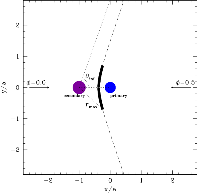
Fig. 7. Schematic view of the geometry of the toy model of the wind interaction zone. The primary star is shown at the origin of the axes, while the secondary is located at x/a = -1 . The shock front is computed according to the formalism of Cantó et al. (1996). Only the thick part of the wind interaction zone (corresponding to a maximum radius r_{\max} from the center of the secondary contributes to the X-ray emission). The angle \theta_{\infty} corresponds to the asymptotic shock cone opening angle. The arrows yield the projections of the line of sight at the conjunction phases onto the orbital plane.
