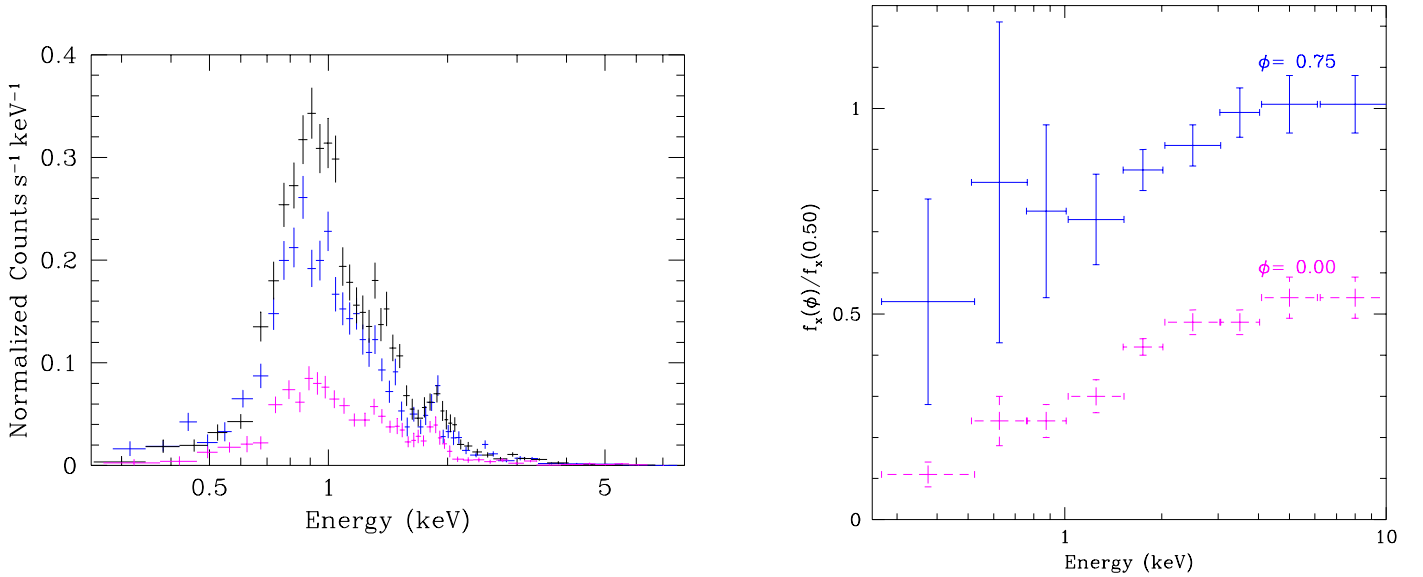
Fig. 2. Left: EPIC-pn spectra of HDE 228766 at the three orbital phases. The black, blue, and magenta symbols stand for phases 0.50, 0.75, and 0.00, respectively. Right: ratio of the observed X-ray fluxes over a series of narrow energy bands with respect to the fluxes at phase 0.5.
