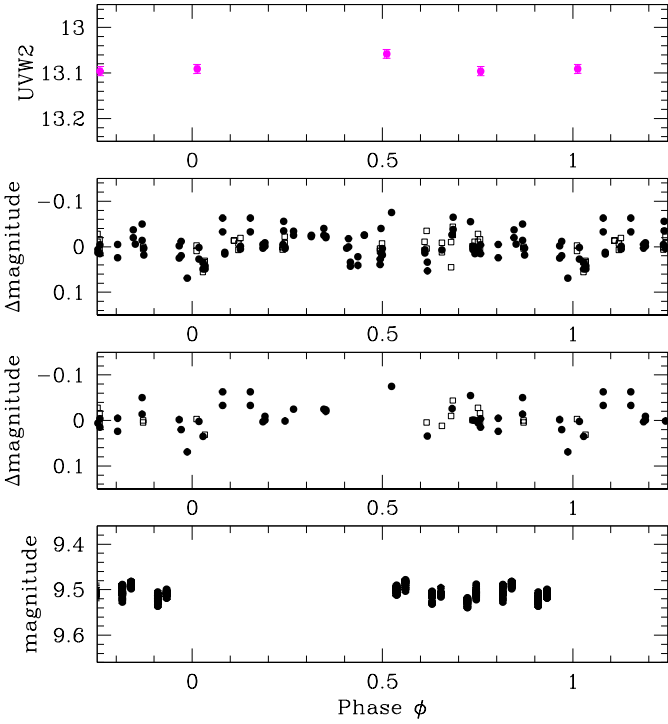
Fig. 6. Top panel: OM light curve of HDE 228766 in the UVW2 filter. Second and third panels from top: NSVS light curve of HDE 228766. Open squares stand for data from Obj. ID 5725284, while filled circles indicate Obj. ID 8495712 in the NSVS database (Woźniak et al. 2004). In the second panel, all 117 data points are shown, including those which were obtained via a deblending procedure. The third panel shows only those 42 data points that remain after rejecting the measurements obtained via PSF deblending. Bottom panel: SuperWASP light curve of HDE 228766.
