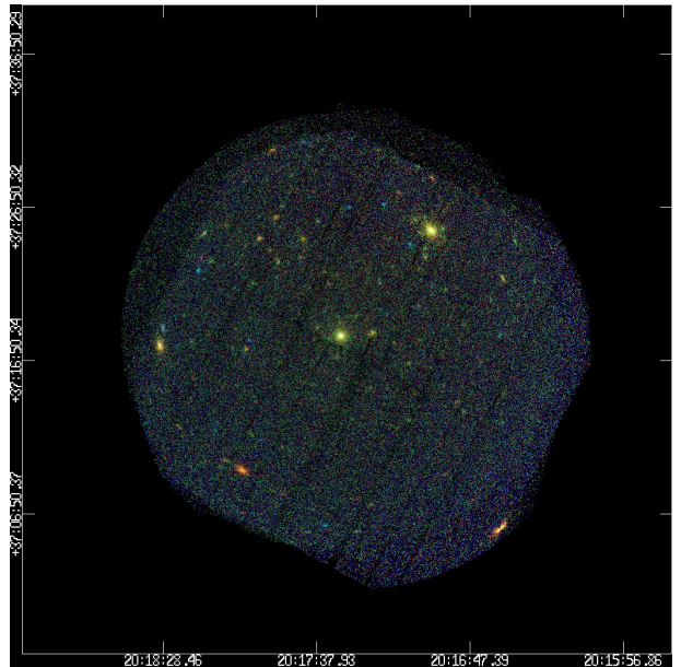
Fig. 1. Energy-coded, three-color X-ray image of the field of view around HDE 228766 built from the EPIC data of the three observations. North is up and east is to the left. The red, green, and blue colors correspond to the photons in the energy ranges of 0.5 – 1.0, 1.0 – 2.0, and 2.0 – 8.0 keV, respectively. The individual images were exposure corrected before they were combined. The bright source to the northwest of HDE 228766 is the Wolf-Rayet binary WR 138 (Palate et al. 2013).
