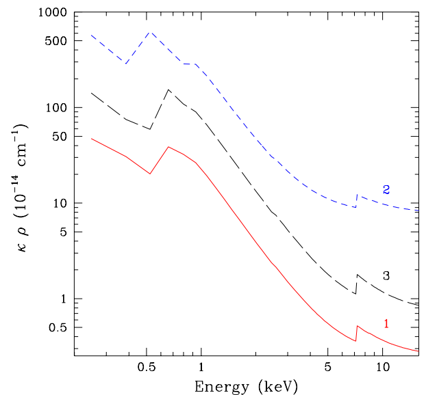
Fig. 3. The product of the wind opacity \kappa(E) and the wind density \rho at 2R_* , as a function of energy for the three model atmospheres. The continuous, short-dashed and long-dashed lines correspond to models 1, 2 and 3, respectively.
