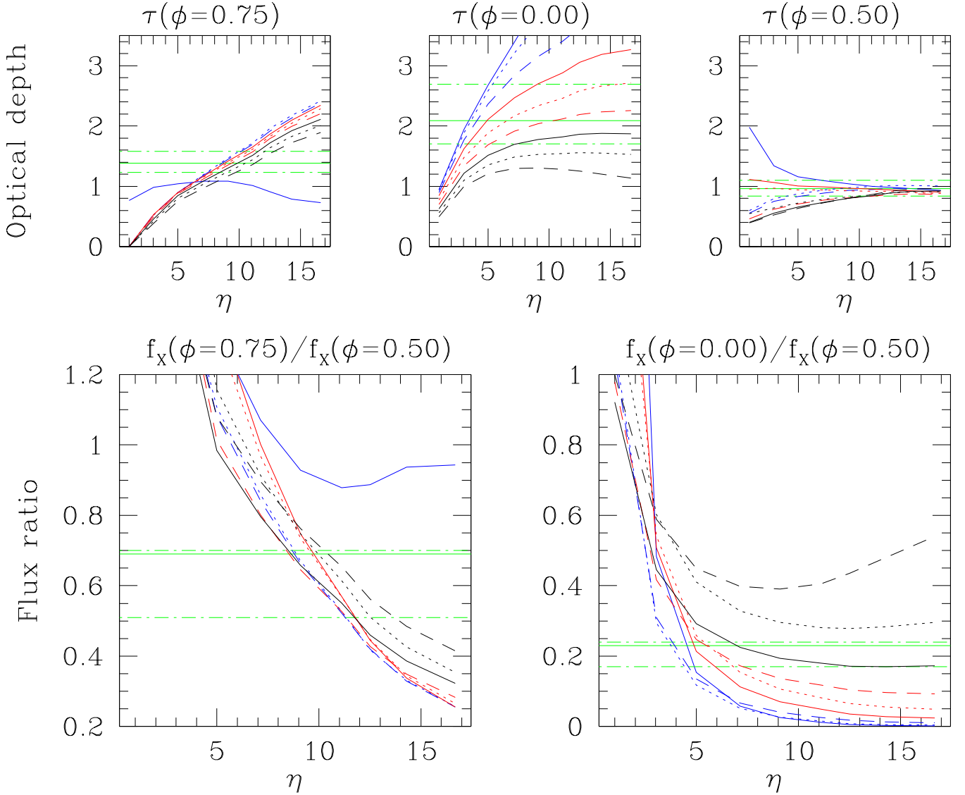
Fig. 8. Output from the toy model for the three optical depths (top panels) and the two flux ratios (bottom panels). The green horizontal lines yield the observed values and their error bars. The blue lines correspond to inclinations of 90, 85 and 80° for the solid, dotted, and dashed lines, respectively. The solid, dotted, and dashed red and black lines yield in turn the results for inclinations of 75, 70, 65°, and 60, 55, 50°, respectively. The model adopted here uses the opacities from Model 2 and assumes \dot{M}_1 = 1.87 \times 10^{-6} M_\odot \text{ yr}^{-1} , v_{\infty,1} = 2245 \text{ km s}^{-1} , r_{\text{max}} = 0.75 a .
