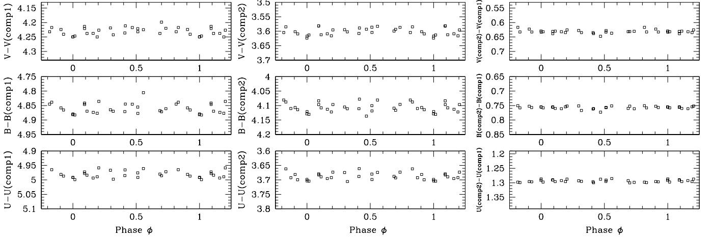
Fig. 5. Same as Fig. 4, but after averaging all the data taken during a specific observing night and retaining only those nights where at least 5 observations had been obtained.
