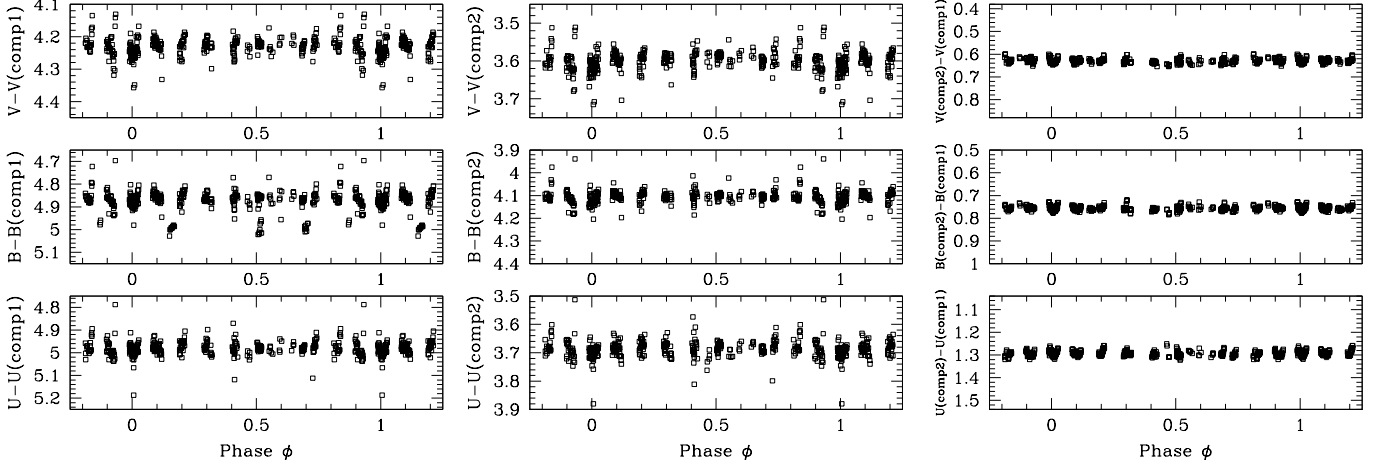
Fig. 4. UBV light curves of HDE 228766 as a function of orbital phase built from our SPM photometric data. The first and second columns of panels correspond to differential photometry with respect to comparison star HD 188892 and HD 193369, respectively. The rightmost column of panels illustrates the difference between the two comparison stars.
