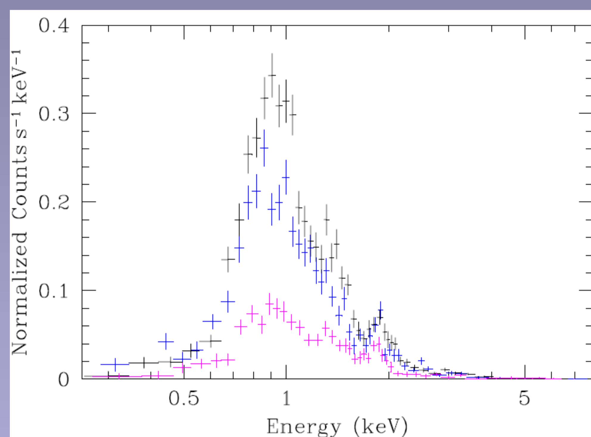
Fig.2: EPIC-pn spectra of HDE228766 at \phi = 0.0 (magenta), \phi = 0.50 (black) and \phi = 0.75 (blue).
