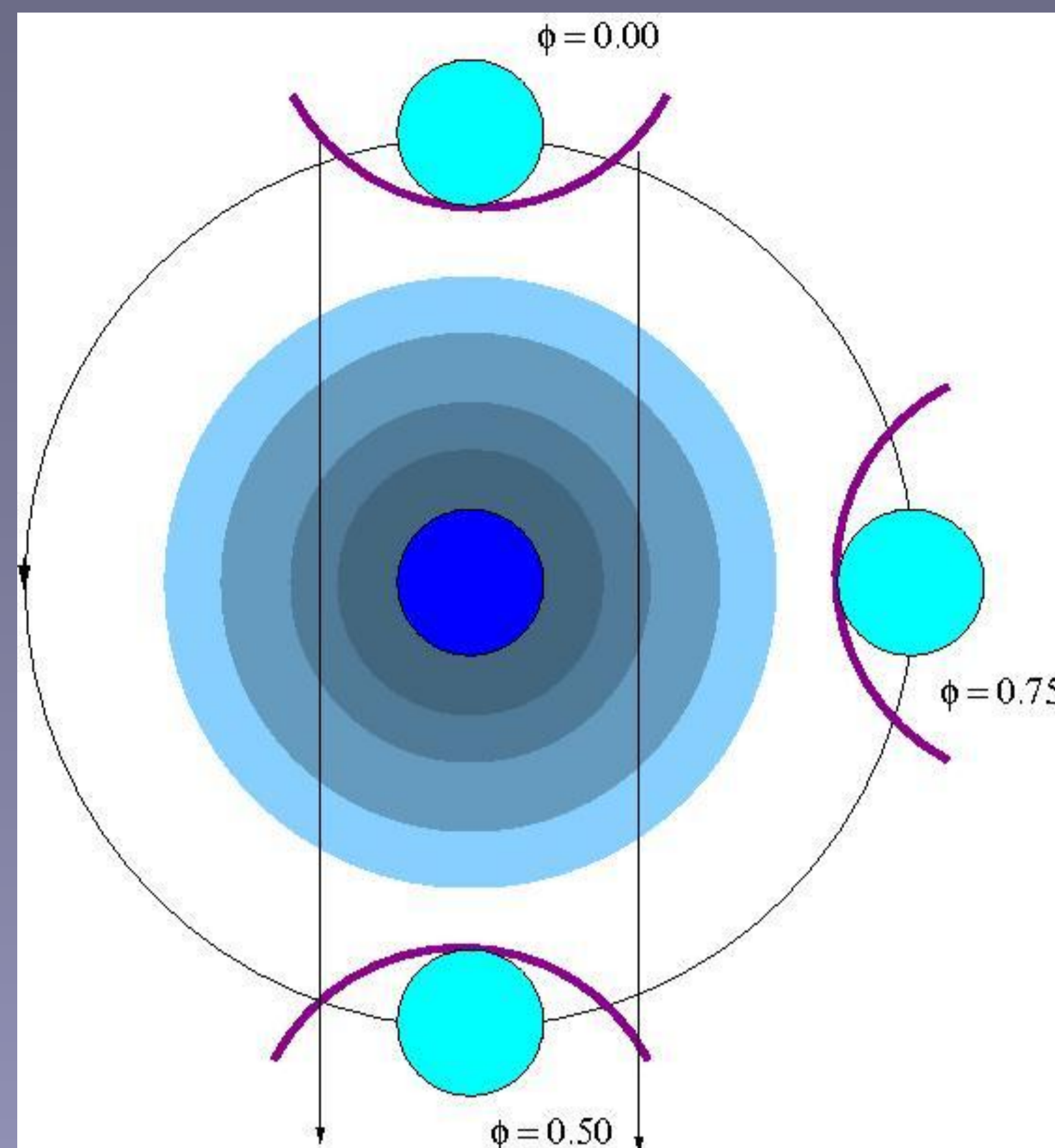
Fig.1, left: schematic illustration of the orbital configuration of the O7 star at the times of the X-ray observations. The observer is at the bottom. Right: combined EPIC image of the FoV around HDE228766. The X-ray spectra of WR138 were analyzed by Palate et al. (2013).
