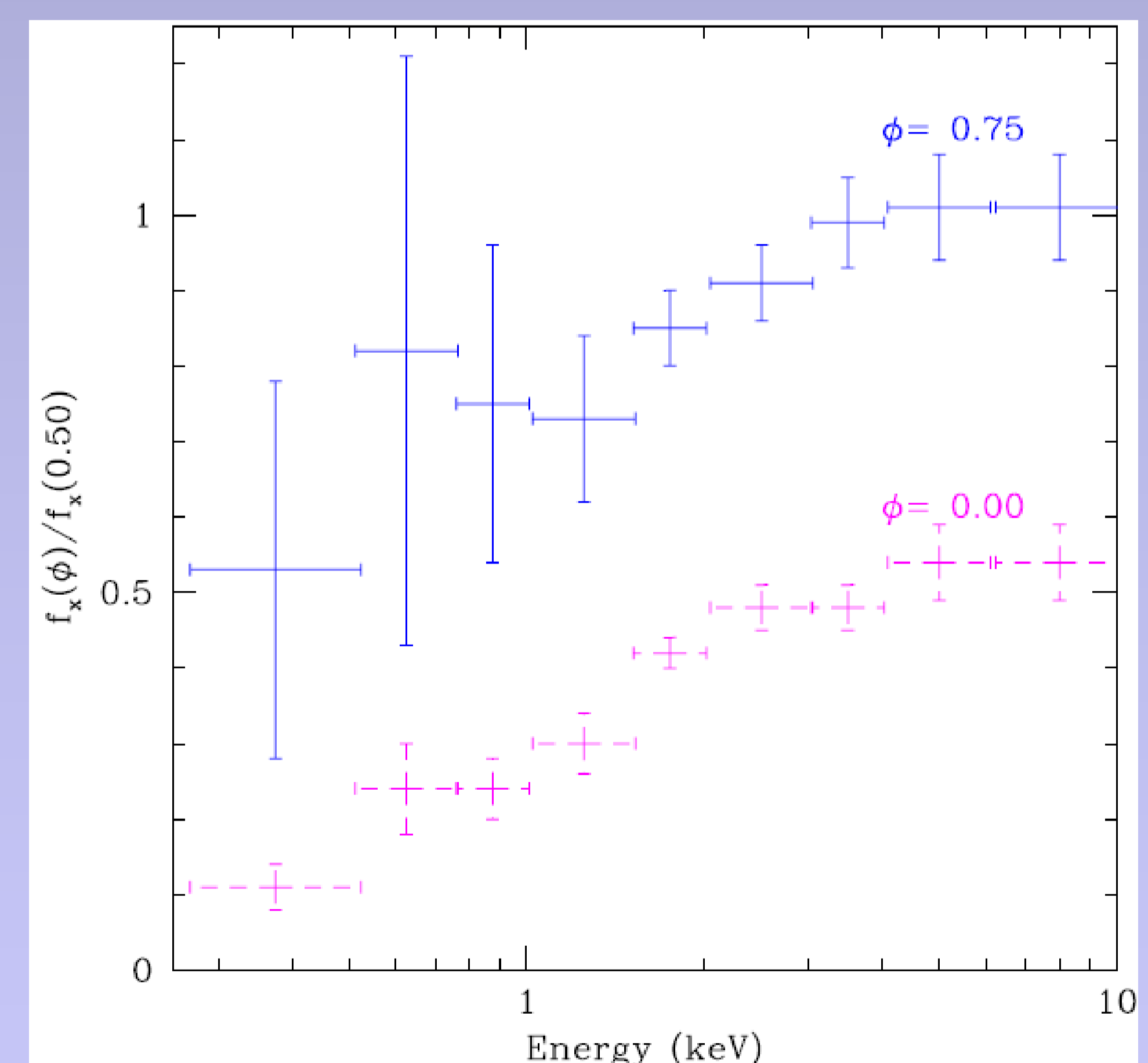
Fig.3: ratio of the observed fluxes over narrow energy bands with respect to those at phase 0.50.
