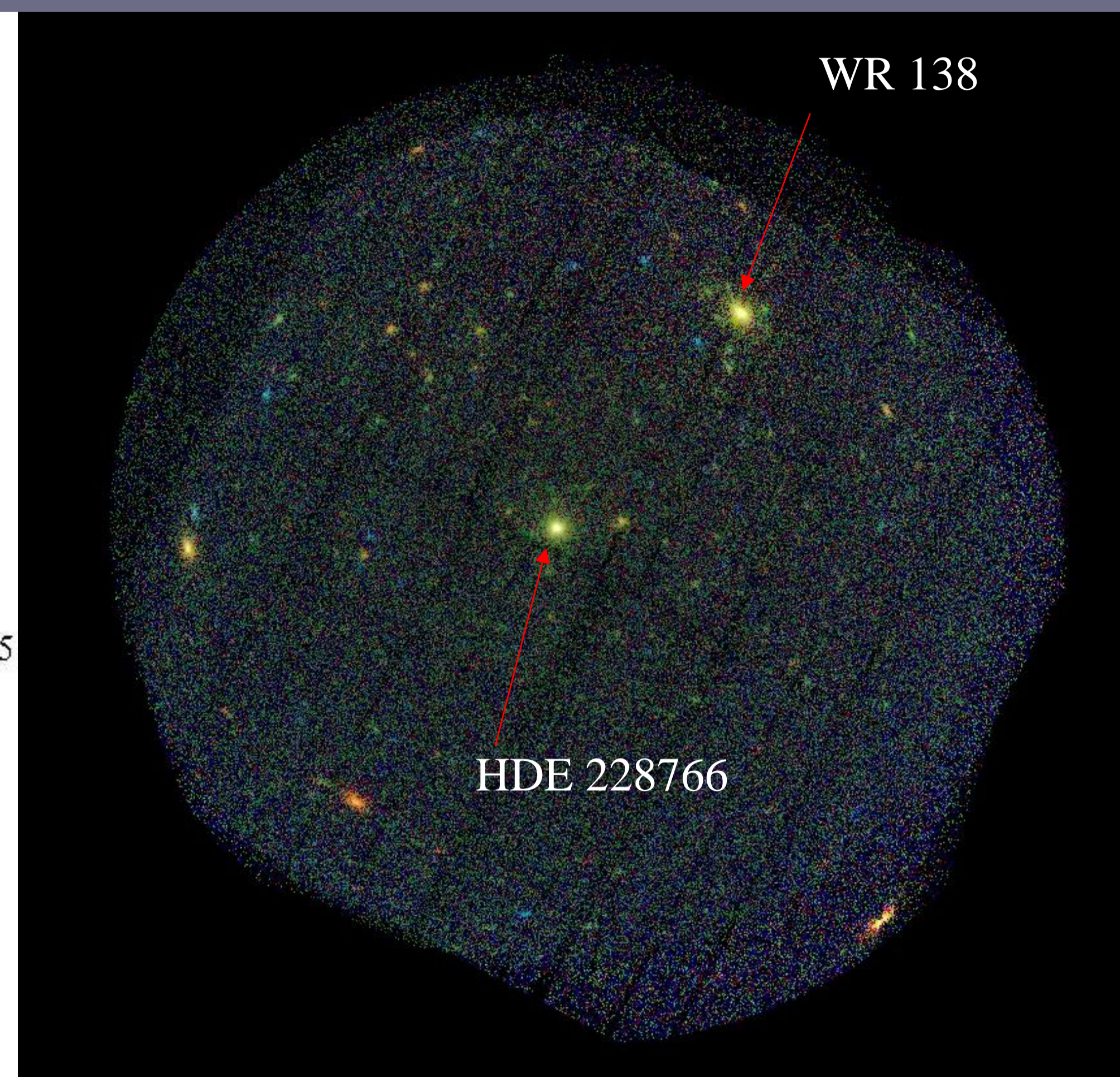
Fig.1, left: schematic illustration of the orbital configuration of the O7 star at the times of the X-ray observations. The observer is at the bottom. Right: combined EPIC image of the FoV around HDE228766. The X-ray spectra of WR138 were analyzed by Palate et al. (2013).
