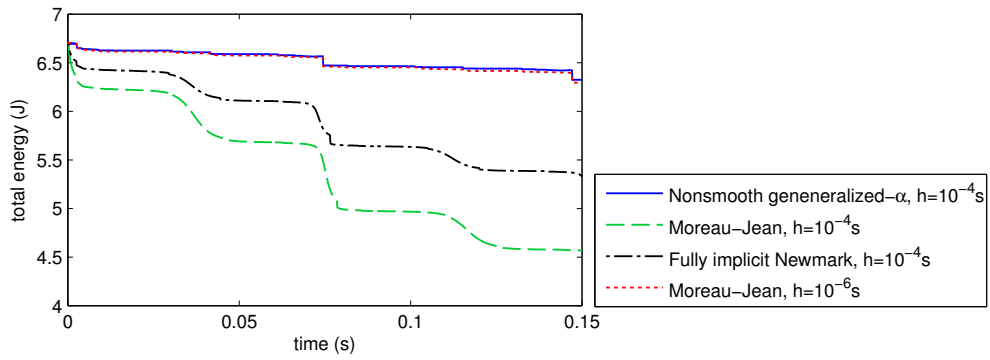
Figure 19: Comparison of different time integration methods for the flexible crank-slider mechanism : (a) crank speed, (b) total energy.
