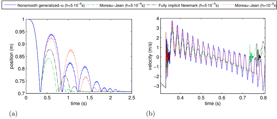
Figure 11: Numerical results for the impact of a flexible rotating beam: (a) position, (b) velocity.
