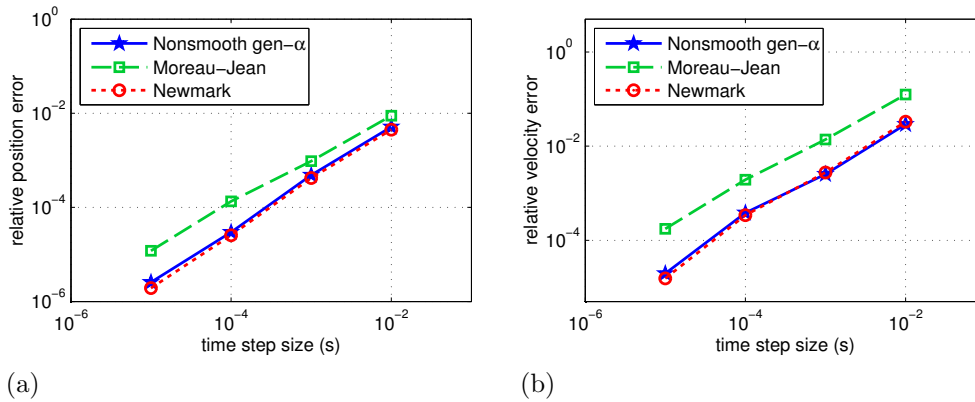
Figure 15: Relative errors on L^1 norm for the bouncing pendulum: (a) position, (b) velocity.
