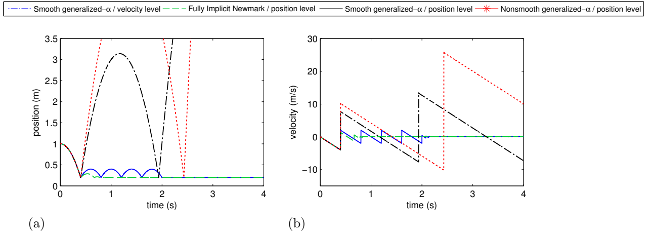
Figure 4: Position and velocity of the bouncing ball vs. time: numerical methods with non consistent response.
