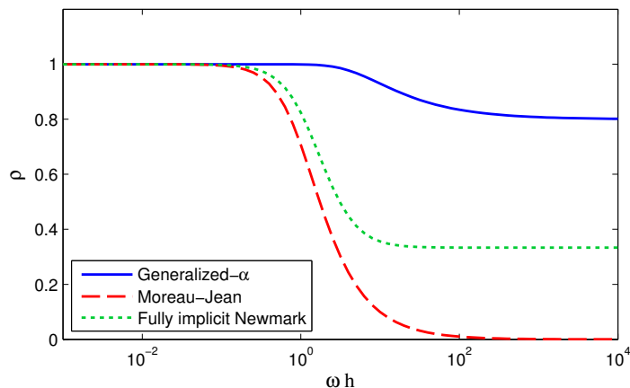
Figure 1: Spectral properties of time integration schemes.
