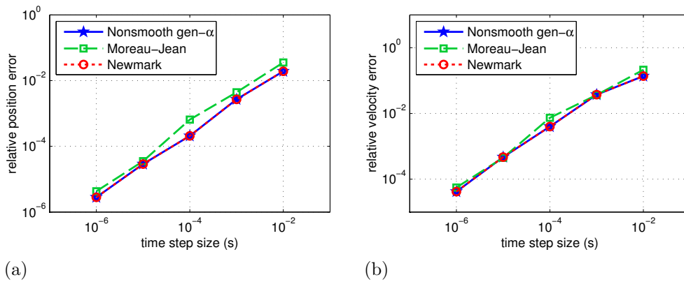
Figure 5: Relative errors on L^1 norm for the bouncing ball: (a) position, (b) velocity.
