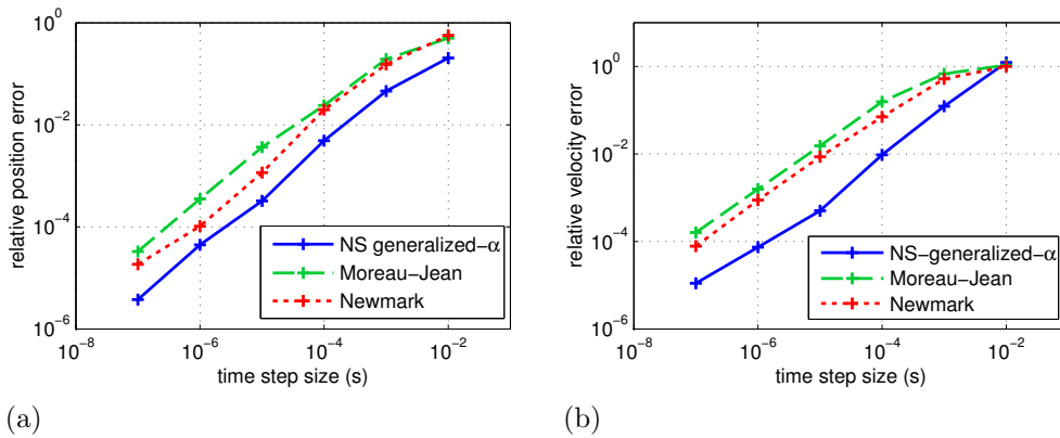
Figure 7: Relative errors on L^1 norm for the bouncing oscillator: (a) position, (b) velocity.
