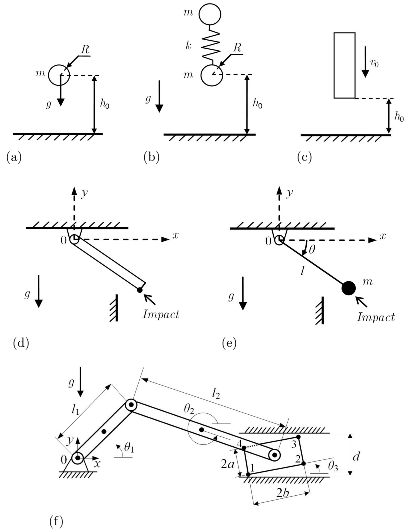
Figure 2: Examples: (a) bouncing ball; (b) linear vertical oscillator; (c) bouncing of an elastic bar; (d) impact of a flexible rotating beam; (e) impact of a rigid pendulum; (f) multiple impacts of a crank-slider mechanism.
