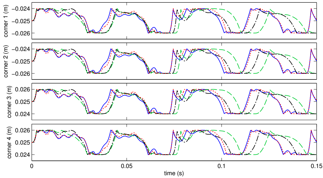
Figure 18: Slider corners' position of the flexible crank-slider mechanism with different time integration schemes : (a) slider corners' position vs. crank revolutions, (b) slider corners' position vs. time.
