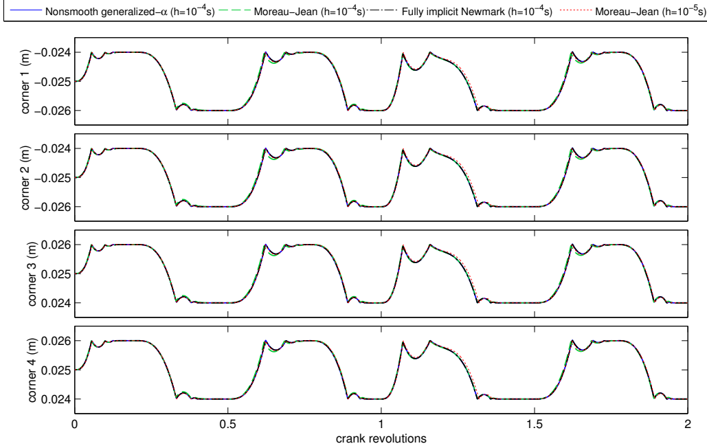
Figure 16: Slider corners' position of the rigid crank-slider mechanism with different time integration schemes.
