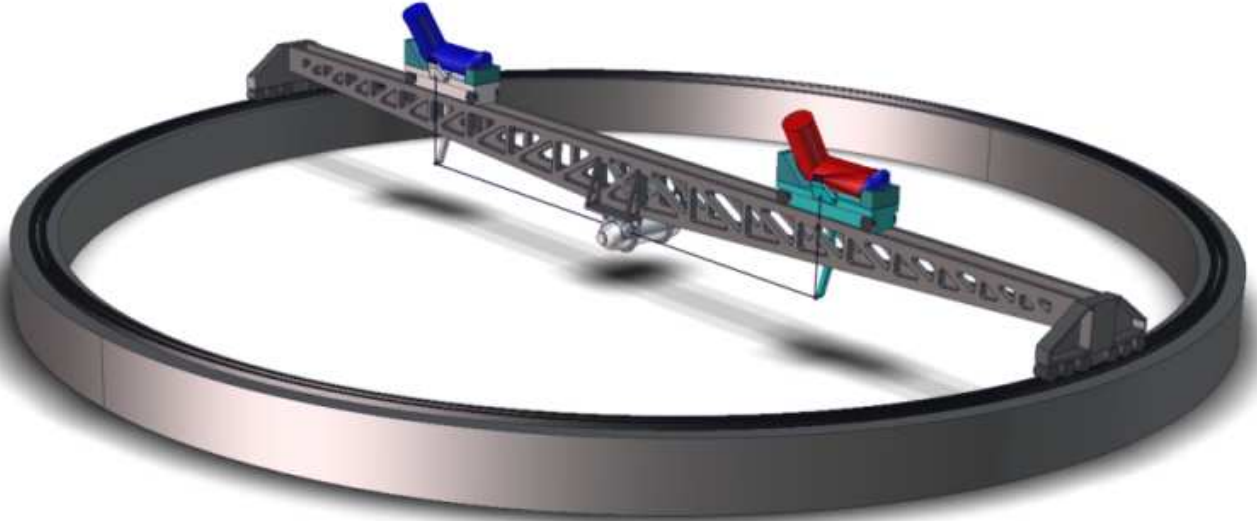
Fig. 1. Overview of the ALADDIN infrastructure. A 40-m rotating truss bearing the siderostats is mounted on a 30-m high structure (not represented). The light beams collected by the two siderostats are fed into off-axis telescopes and routed towards the nulling instrument cryostat by fixed relay optics (only five reflections outside the cryostat).
