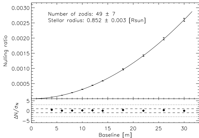
Fig. 5. Simultaneous fit of the stellar radius and the exozodiacal density level using ten 30-min observations of a K0V star at 5 pc (actual radius of 0.85R_{\odot} ), surrounded by a 50-zodi disc. The nulling ratio is computed as the ratio between the destructive and constructive outputs of the beam combiner. The contribution of instrumental stellar leakage to the nulling ratio has been subtracted from this data using the same procedure than elaborated for GENIE: the observation of a calibration target of similar type and distance, but without circumstellar material.
