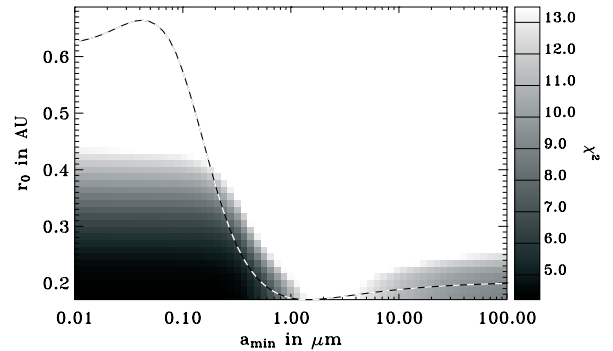
Fig. 5. Map of the \chi^2 as a function of minimum grain size a_{\min} and inner radius r_0 , obtained by fitting the circumstellar disk model of Augereau et al. (1999) to the SED data of Table 4. We have assumed a surface density power-law \Sigma(r) \propto r^{-4} and a grain size distribution dn(a) \propto a^{-3.7} da , with a maximum size of 1500 \mu\text{m} . In this simulation, the disk is composed of 50% amorphous carbons and 50% glassy olivines (see text). The dashed line represents the distance at which sublimation happens for dust grains of a given size (isotherm T = 1700 K). The axis labels should therefore read “ a in \mu\text{m} ” and “sublimation radius in AU” for this curve.
