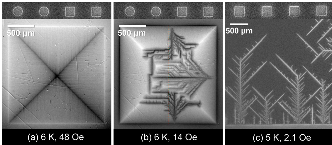
FIG. 3. MO images taken for sample Nb-I, with circular (left side) and square (right side) ADs, taken at (a) T = 6 K and H = 48 Oe, showing isotropic flux penetration; and (b) at T = 6 K, for H = 14 Oe (after decreasing from H = 48 Oe), revealing different morphologies depending on the AD geometry. (c) MO image for sample Nb-II (square lattice of square ADs) taken at T = 5 K and H = 2.1 Oe, showing avalanches with the Christmas Tree morphology.
