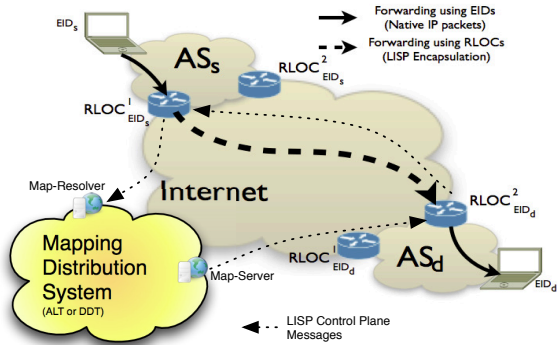
Fig. 1. LISP data and control plane packet forwarding sequence.
