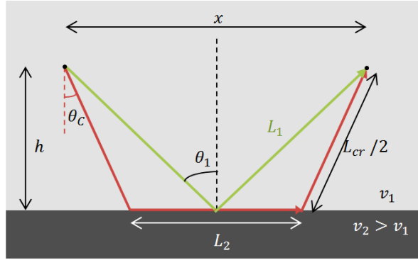
Figure 33 : Representation of the ray propagation of a lateral wave.
