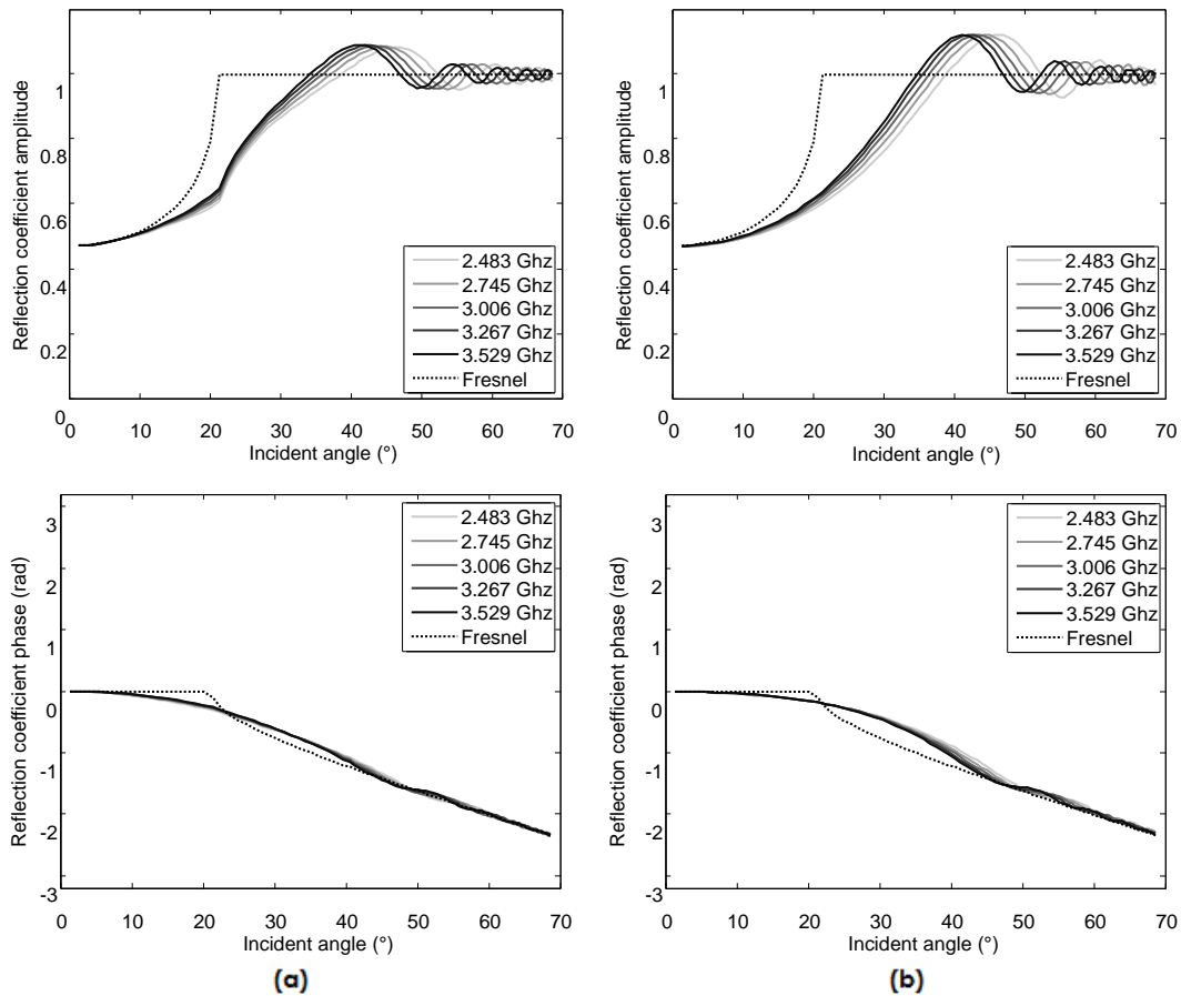
Figure 35 : Amplitude and phase of the global reflection coefficients with \epsilon'_{r1} = 7.7 , \epsilon'_{r2} = 1 and h = 10 \text{ cm} : (a) obtained with the spherical waves formulas; (b) obtained through the analysis of 3D numerical simulations.
