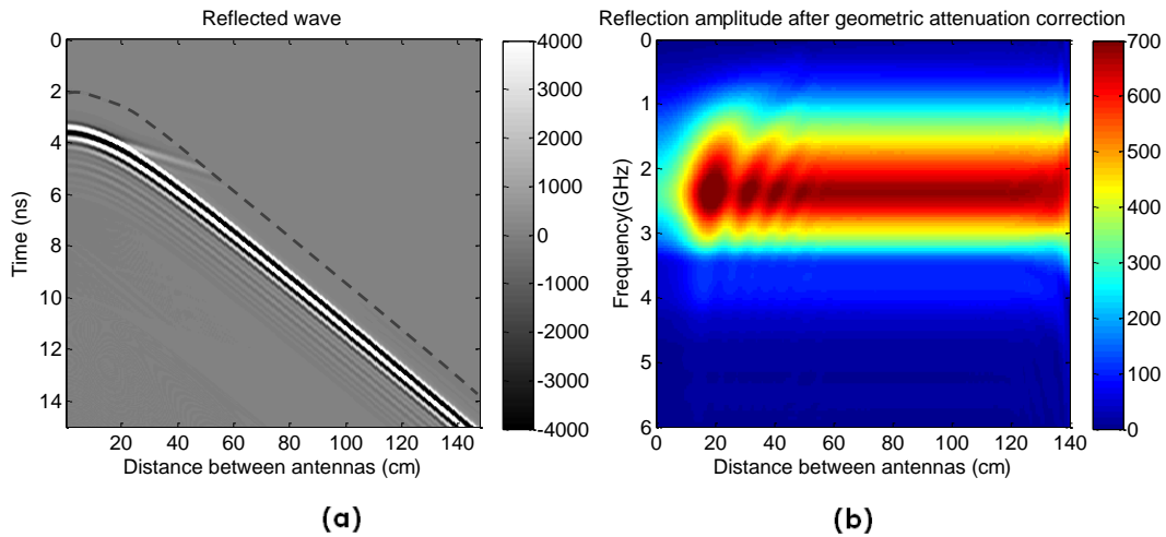
Figure 94 : (a) Radargram and (b) frequency amplitude of the reflection measured over a simple concrete-air interface, after correction of the geometric attenuation.
