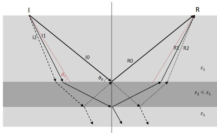
Figure 43 : Thin layer reflection of a spherical wave for incident angle larger than the critical angle.
