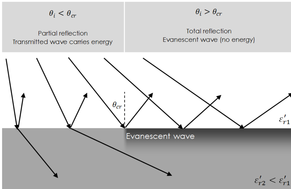
Figure 30 : The evanescent wave appears when the incident angle \theta_i is larger than the critical angle.
