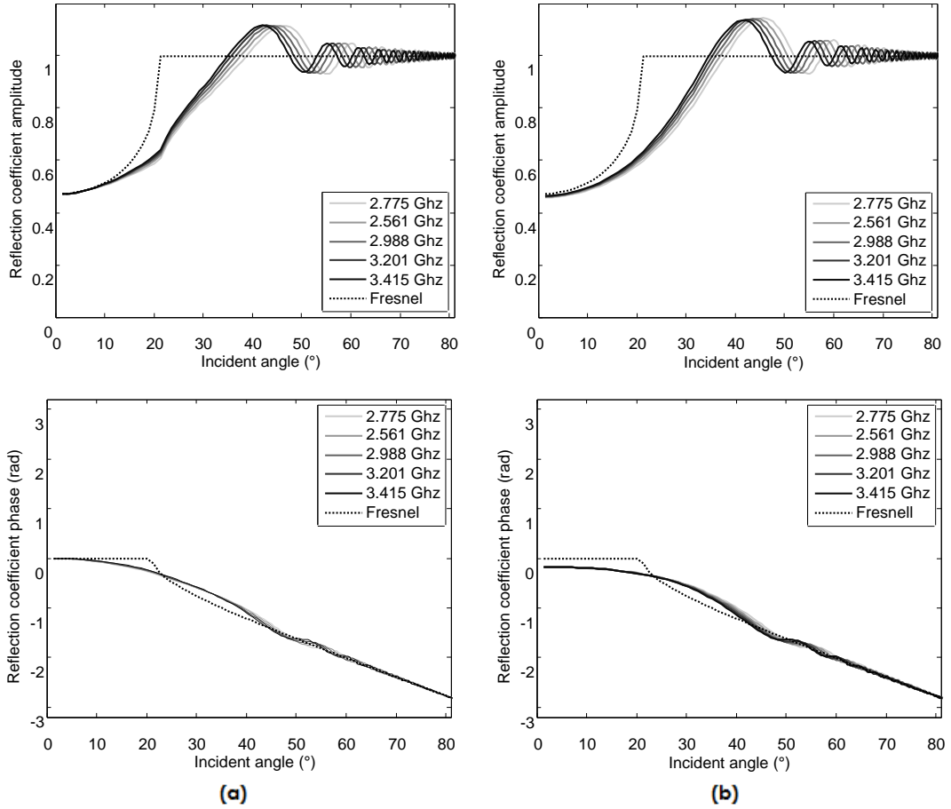
Figure 177 : Amplitude and phase of the global reflection coefficients with \varepsilon'_{r_1} = 7.7 , \varepsilon'_{r_2} = 1 and h = 10 \text{ cm} ; (a) obtained with the modified formulas taking into account the spherical waves reflection and the lateral; (b) measured through the analysis of numerical 2D simulations.
