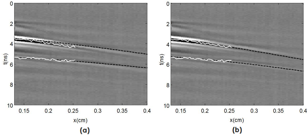
Figure 84 : Best approximation of the CMP reflections (represented by the dashed line) with h unknown (a) based on the second reflection only; (b) based on the two first reflections.
