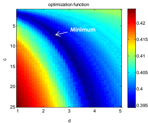
Figure 106 : Optimization function for the coefficient c and d of the amplitude function of the first terms with spherical formula. The theoretical reflection coefficient curves obtained for 5, 7, 9 and 11 cm with this formula are compared to the reflection coefficients measured in 2D numerical simulations.
