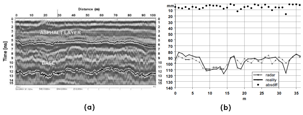
Figure 11 : (a) Example of road survey displaying the interfaces between the different layers [47]. (b) Comparison of the asphalt thickness estimated by GPR measurements to the real one [45].
