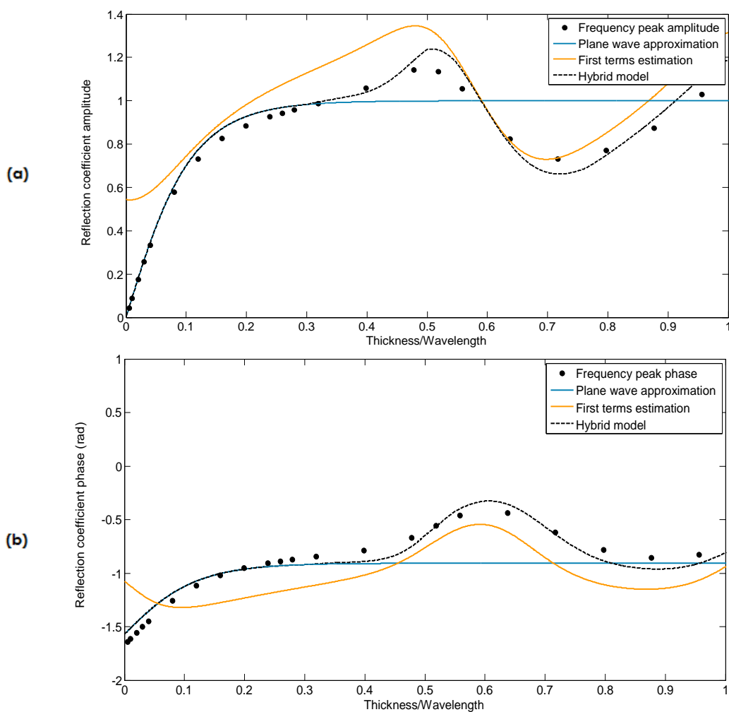
Figure 139 : (a) Amplitude and (b) phase of air thin layers reflection coefficients, depending on the thickness-to-wavelength ratio, for a post-critical incidence. Comparison of numerical test results and analytical curves.
