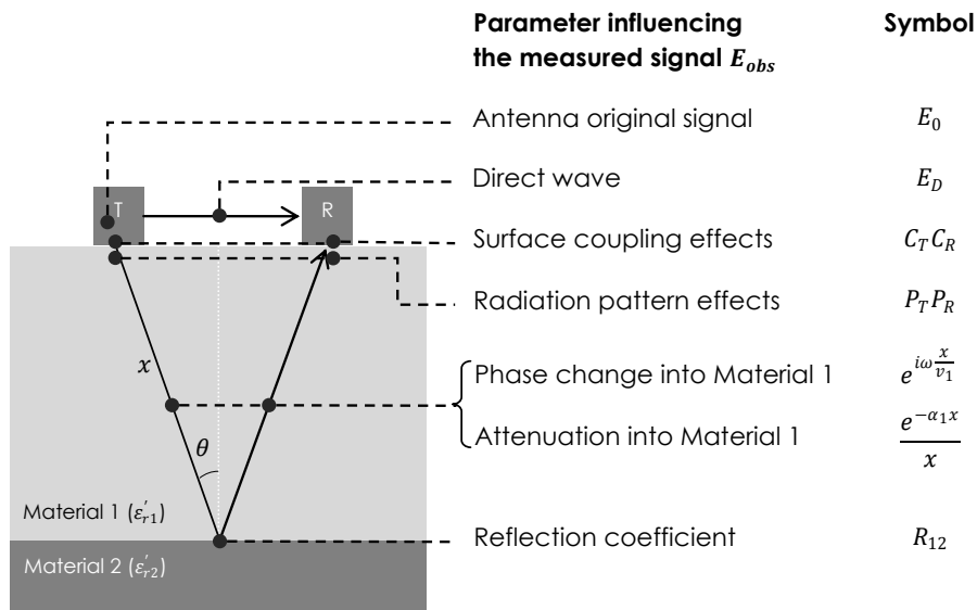
Figure 46 : Parameters influencing the electric field E_{obs} measured over an interface buried in an homogeneous material.
