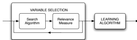
Figure 1.3: Variable selection is a preprocessing step of learning composed of a search algorithm combined with an evaluation function.
