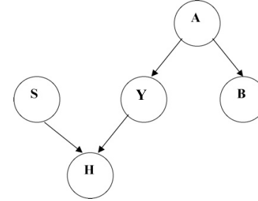
Figure 4.1: Artificial Bayesian network describing the interaction of variables : abnormal cellular activity (A), cancer (Y), blood marker (B), headache (H) and sinus infection (S).
