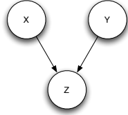
Figure 2.4: Graphical representation of the relationships between the variables of Example 2.2
