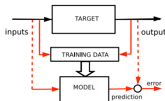
Figure 1.1: Data-mining through supervised learning consists in building a model from data in order to predict a target function.
