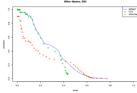
Figure 4.6: PR-curves for the RS3 dataset using Miller-Madow estimator. The curves are obtained by varying the rejection/acceptation threshold.
