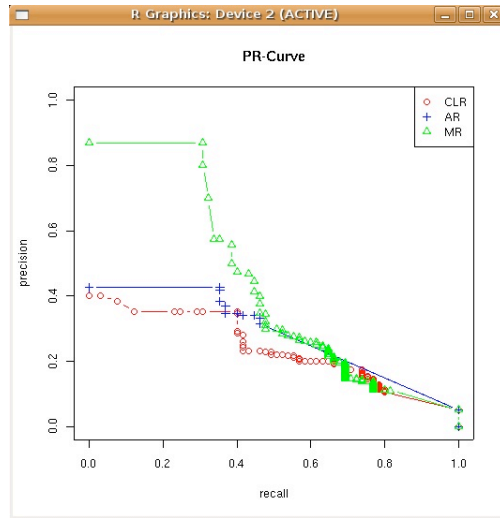
Figure 4.4: Precision-Recall curves plotted with SHOW.PR(TABLE)
