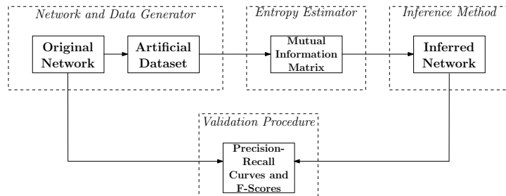
Figure 4.5: An artificial microarray dataset is generated from an original network. The inferred network can then be compared to this true network.
