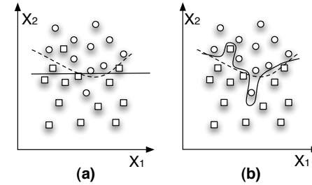
Figure 2.6: The output Y can take two values: square or bullet, the continuous line is the model, the dashed line is the target function. In (a) a linear model that underfits the target function. In (b) a complex non-linear model that overfits the target function (fits the noise).
