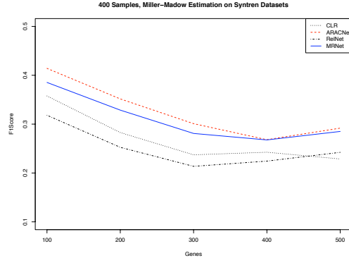
Figure 4.8: Influence of the number of variables on accuracy ( SynTReN SV datasets, Miller-Madow estimator).
