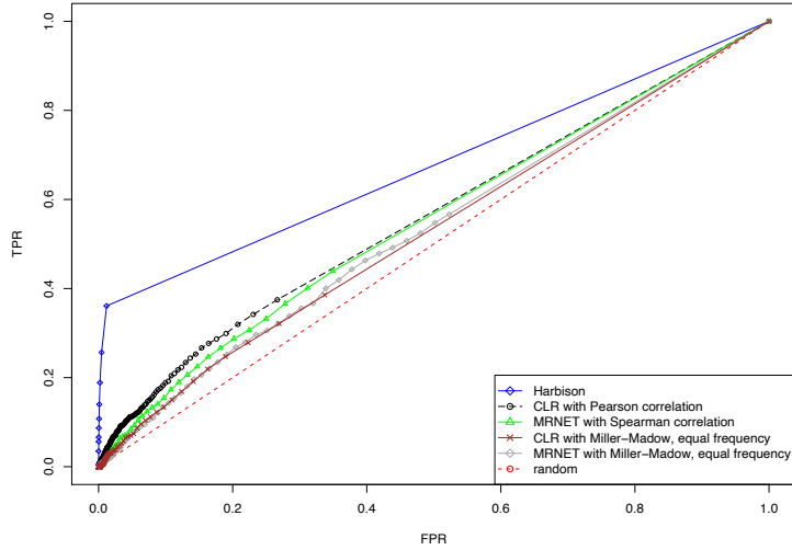
Figure 4.13: ROC curves: Harbison network, CLR combined with Pearson correlation, MRNET with Spearman correlation, CLR combined with the Miller-Madow estimator using the equal frequency discretization method, MRNET with Miller-Madow using equal frequency discretization and random decision.
