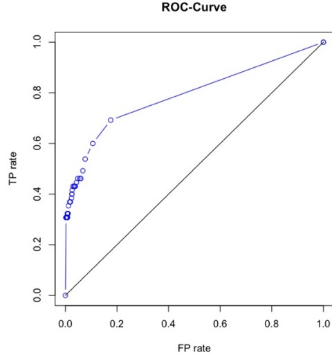
Figure 3.3: Example of ROC curves (generated with the R package 'minet' [89])
