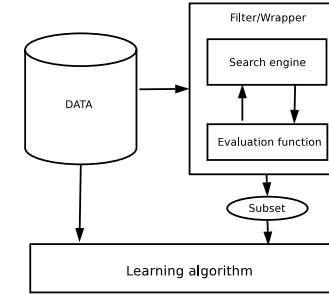
Figure 3.2: principle of a filter/wrapper approach
