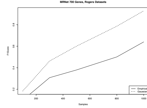
Figure 4.10: Influence of mutual information estimator on MRNET accuracy for the two MIM estimators ( sRogers RS datasets).
