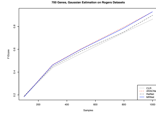
Figure 4.7: Impact of the number of samples on accuracy ( sRogers RS datasets, Gaussian estimator).
