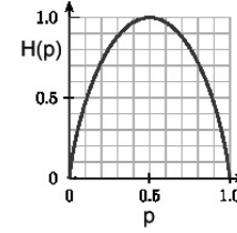
Figure 2.1: H(p) as a function of p (Bernoulli distribution)
