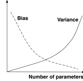
Figure 2.5: Bias-variance dilemma
