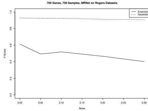
Figure 4.9: Influence of the noise on MRNET accuracy for the two MIM estimators ( sRogers RN datasets).
