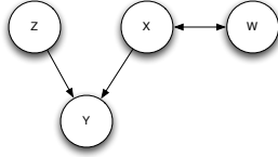
Figure 2.3: Graphical representation of the relationships between the variables of example 2.1
