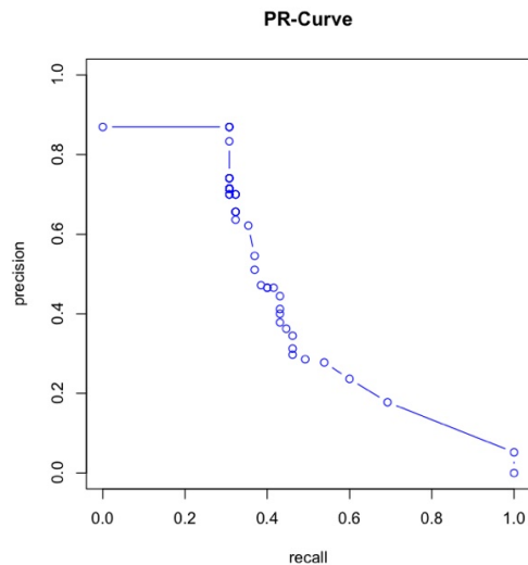
Figure 3.4: Example of PR curves (generated with the R package 'minet' [89])
