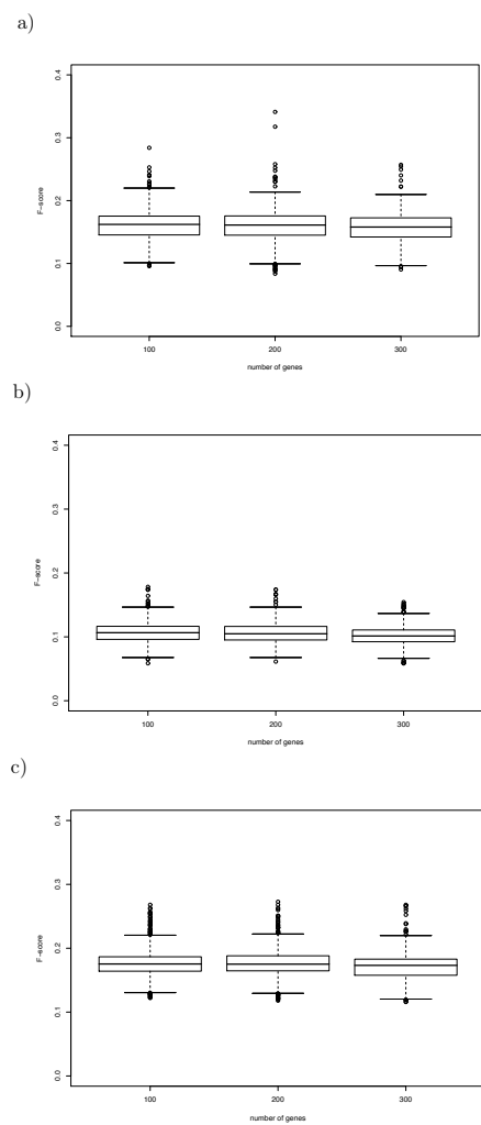
Figure 4.11: Mean F-scores and standard deviation with respect to number of genes, for all 10 repetitions with additive Gaussian noise and no missing values. a) MRNET, b) ARACNE and c) CLR
