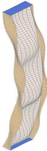
Figure 2. Geometrical imperfections
