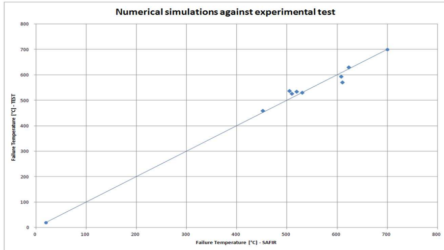
Figure 3. Comparison between experimental tests and numerical simulations
