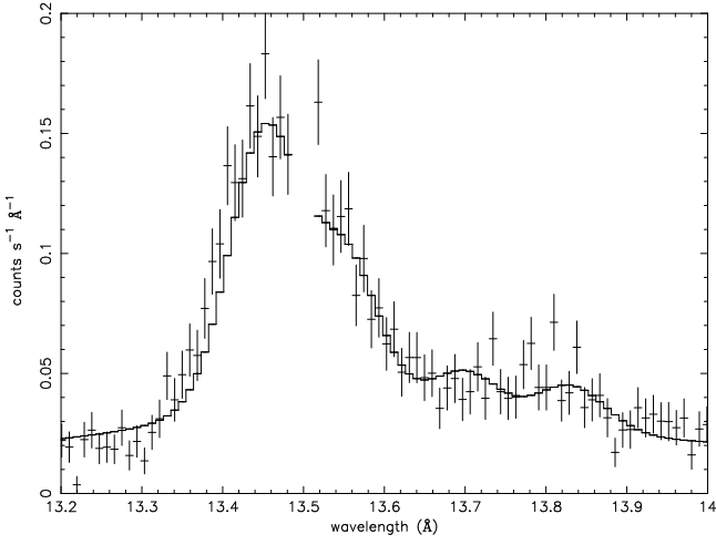
Fig. 4. The Ne IX triplet with best fit model. Only RGS 2 data are shown for clarity, but both were used in the fit. There is also a Fe XVII line at 13.825 Å. The rest wavelengths of the three lines are at 13.45 Å (r), 13.55 Å (i), and 13.70 Å (f).
