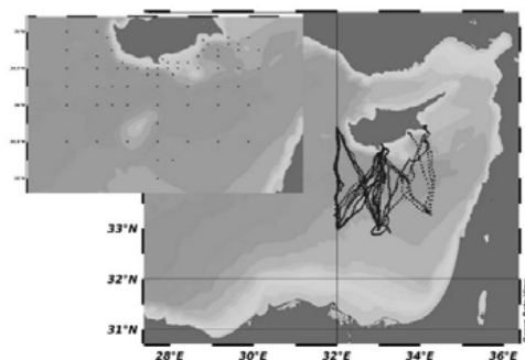
Fig. 1. Location map of standard Cyprus Oceanography hydrographic stations (zoom) and Cyprus glider fleet missions (2009-2012).
