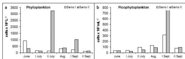
Fig. 1. Phytoplankton (a) and picophytoplankton (b) abundances (cells \times 10^3 L -1 and cells \times 10^3 mL -1 , respectively) in Seno I and Seno II in summer 2008.
