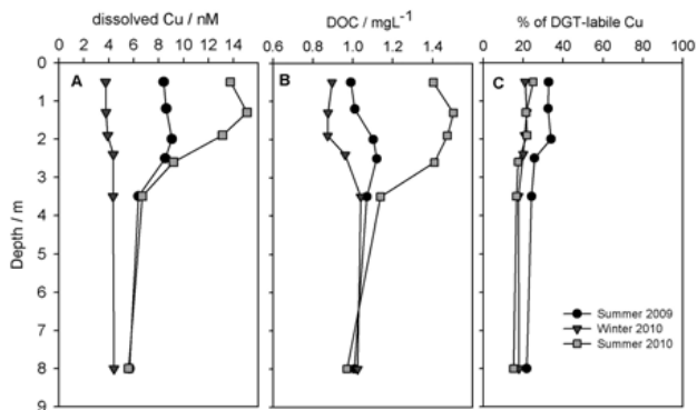
Fig. 1. Dissolved Cu, DOC and percentage of DGT-labile Cu at a "clean" site
