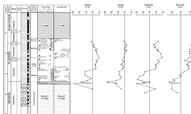
Fig. 1. Calcareous plankton biostratigraphy and stable isotope compositions of calcite and dolomite along the Site 225 stratigraphic sequence
