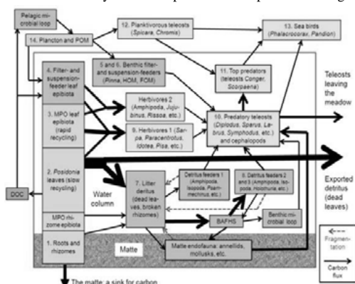
Fig. 1. Conceptual model of the functioning of the Posidonia oceanica ecosystem in the North Western Mediterranean Sea (C.F. Boudouresque, original figure; modified from [1])
