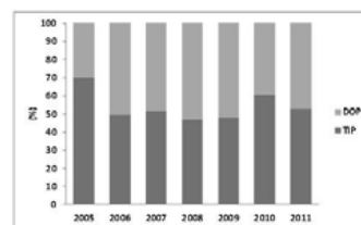
Fig. 2. The percentage contribution of phosphorus species to TDP during the years 2005–2011.
