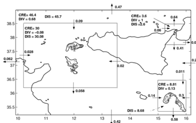
Fig. 2. Model predicted distribution of the depth integrated conversion rate from the K_1 surface to internal tide. Integrated baroclinic energy flux across the bounding transects is given in MW. Conversion (CRE), dissipation (DIS) and flux divergence are in MW
