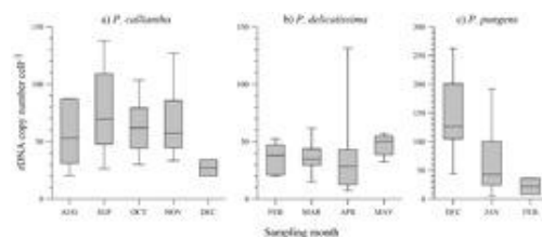
Fig. 1. The rDNA copy number per cell of northwestern P. calliantha , P. delicatissima and P. pungens strains determined by qrt-PCR and sampling period.
