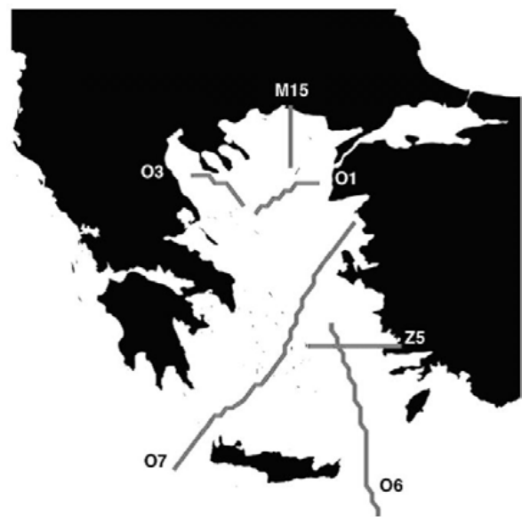
Fig. 1. Map of selected transects to simulate hydrologic data unfortunately not measured.
