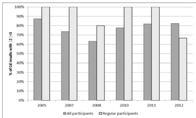
Fig. 1. Percentage of results ( |Z| < 3 ) reported for Cd in MED POL PTs:
