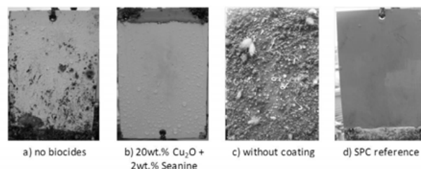
Fig. 2. Pictures of panels coated a) with a FRC/SPC hybrid coating containing no biocides, b) with a FRC/SPC hybrid coating containing 20wt.% of \text{Cu}_2\text{O} and 2wt.% of Seanine 211, c) panel without coating and d) panel coated with a commercial SPC reference, after 7 months of static immersion in the Toulon bay. Fouling organisms were easy removed using a wet sponge at the top of the panel a).
