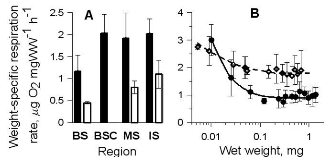
Fig. 1. Respiration rates of active and narcotized (white bars) females from the Black (BS), Marmara (MS), Ionian (IS) Seas and of the Black Sea females (BSC) reared in the laboratory at 18°C and 38 psu (A). Ontogenetic changes of respiration rate at 20°C in Calanus euxinus from the Black (•) and Marmara (◇) Seas (B).
