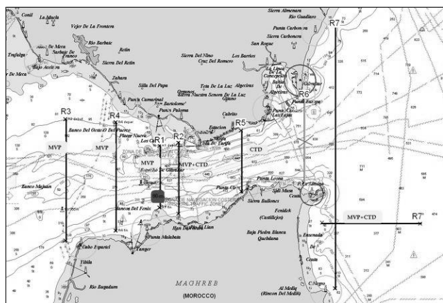
Fig. 1. Map of the sampling during the HydroChanges Gibraltar campaign in July 2012.
