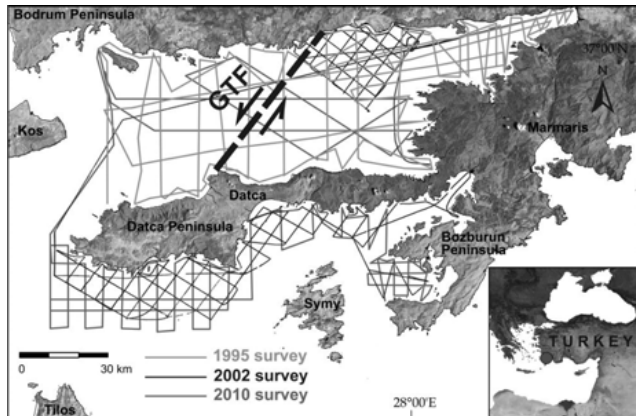
Fig. 1. The location map of study area and seismic lines. GTF: Gökova Transfer Fault.
