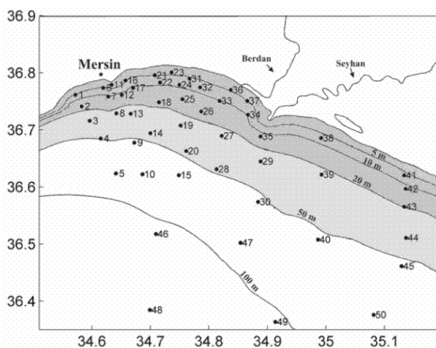
Fig. 1. Locations of sampling stations visited in the Mersin Bay shelf zone
