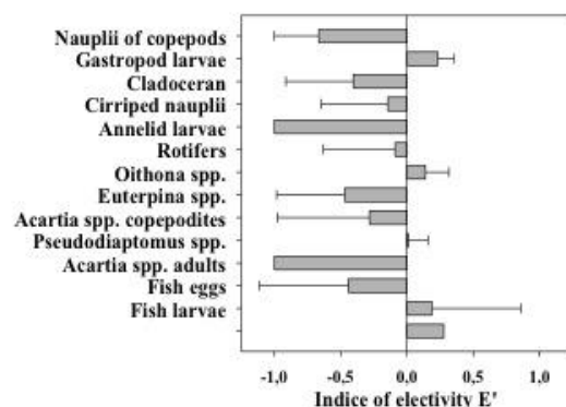
Fig. 2. Indices of electivity E' for each taxa present on the natural zooplankton assemblage.
