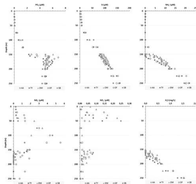
Fig. 2. Nutrient concentrations of Black Sea water column
