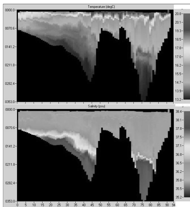
Fig. 2. MVP series of 94 CTD profiles across the R3 transect (from North (left) to South (right)).
