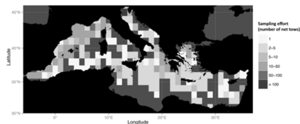
Fig. 1. Copepod data set and sampling effort. The map indicates the spatial coverage of our copepod observation data set. The number of sampling tows projected on a rectangular grid of 1° is also indicated
