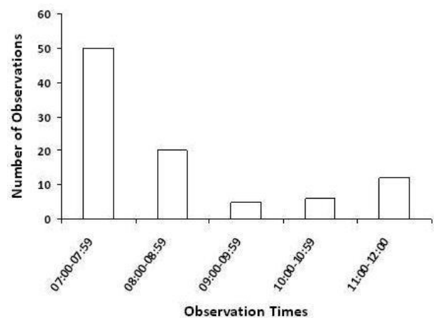
Fig. 2. Number of Sandbar Shark by observation times.
