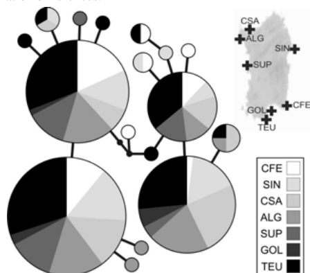
Fig. 1. Haplotype network of COI sequences of O. vulgaris from Sardinia, pie charts are drawn proportionally to the number of sequences.
