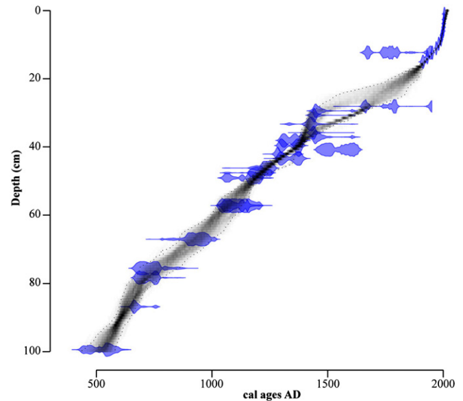
Fig. 2. Age-model produced by BACON software (Blaauw et al., 2011) coupling both ^{14}\text{C} and ^{210}\text{Pb} results. Age-models are based on 50 1-cm thick sections of linear accumulation, with a degree of memory between each section. Grey-scales indicate all likely age–depth models, and dotted lines indicate the 95% confidence ranges. Shapes show calendar age distributions of individual dates (calibrated distributions for the ^{14}\text{C} dates).
