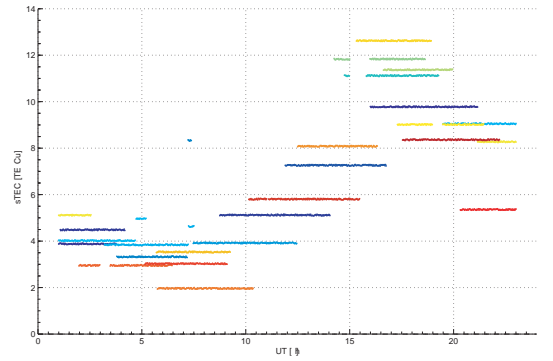
Figure 1: Example of sTEC differences for Brussels station on January 1 st , 2002
