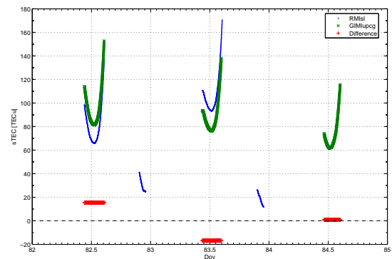
Figure 4: sTEC data and differences for Brussels station between March 23 rd to 25 th , 2002 for PRN 2
