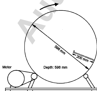
Fig. 1. Principle of the briquette durability tester.
