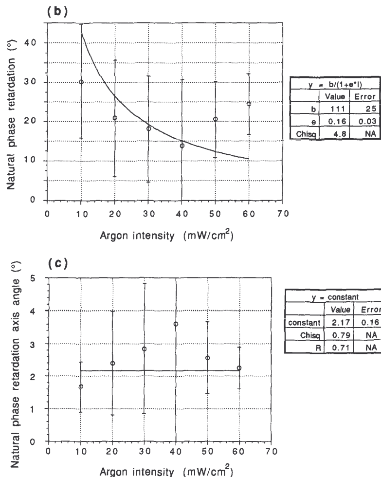
Fig. 6. The plots obtained by fitting in the photoinduced birefringence experiments versus the argon polarisation angle, we obtain a triplet of parameters: \Delta , \Gamma , \varphi . The figures show the plot of these parameters versus the argon intensity for an argon polarisation angle fixed at 40^\circ according to the HeNe polarisation axis. In the three cases, the curve fit is deduced from our model. Inset: fit function and parameter values. (a) Photoinduced phase retardation r versus argon intensity. (b) Natural phase retardation \Delta versus argon intensity. (c) Axis angle \varphi of the natural birefringence versus argon intensity.
