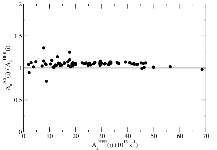
Fig. 6. Comparison of Auger widths ( 10^{13} \text{ s}^{-1} ), A_a(i) , calculated by HFR and AUTOSTRUCTURE (AS). Widths greater than or equal to 10^{13} \text{ s}^{-1} have been retained. A straight line of equality has been drawn.
