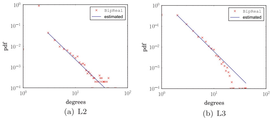
Fig. 15. Frequency distribution of degrees and PDF of estimated distribution, for degrees above or equal to x_m .
