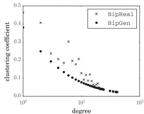
Fig. 10. Degree correlation.
