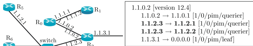
Fig. 1. mrinfo example.
