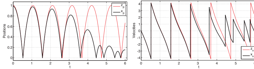
Figure 8.33: Simulation of the destabilizing effects of the linear tracking controller for the hammer example. Left plot: positions; Right plot: velocities. Reference hammer: red; controlled hammer: black.
