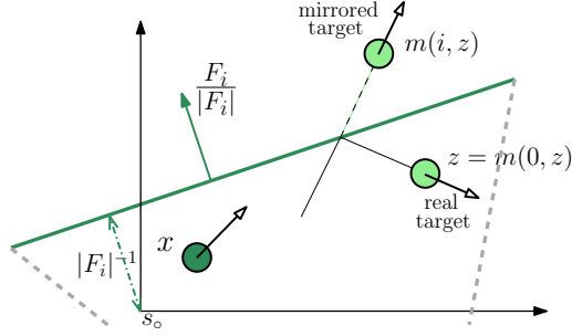
Figure 8.38: The triangular region \mathcal{F} and the mirror of the target z with respect to one wall.
