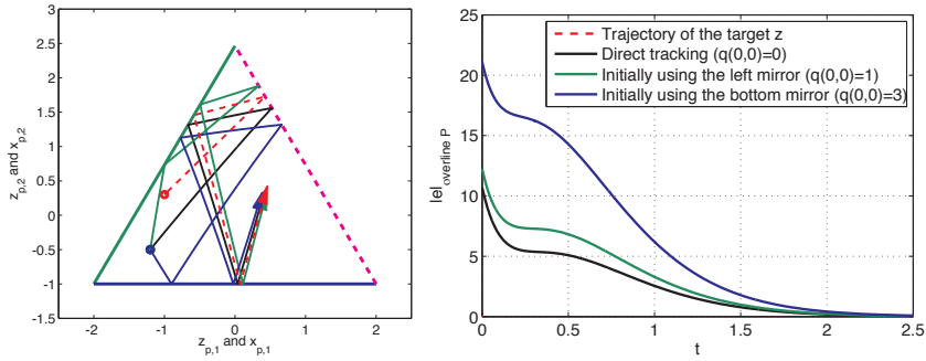
Figure 8.40: Trajectories of the hybrid tracking algorithm in a triangular region (left) and evolution of the generalized error (right).
