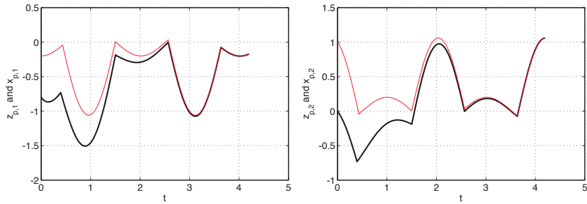
Figure 8.36: Positions (left) and velocities (right) of the Newton cradles for q(0, 0) = 0
