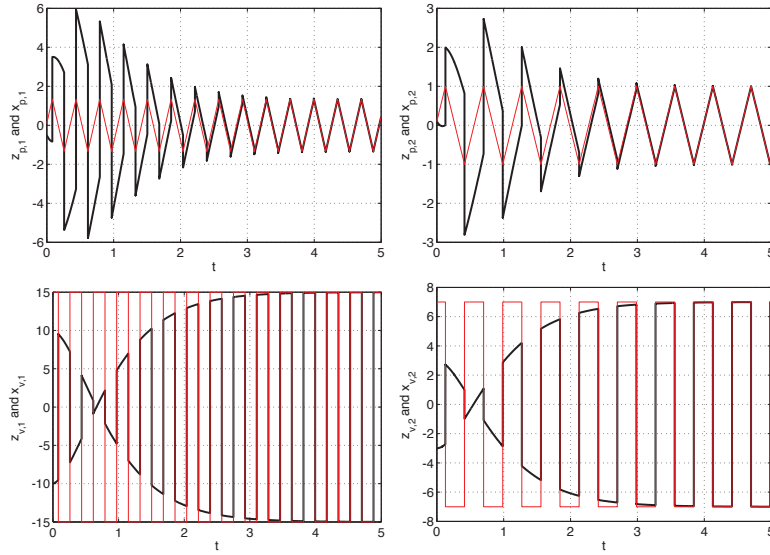
Figure 8.42: Simulation of the hybrid observer on a planar example. The upper graphs show the positions while the lower graphs show the velocity. Reference:red, observer: black.
