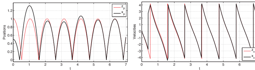
Figure 8.34: Simulation of the hybrid tracking controller for the hammer example. Left plot: positions; Right plot: velocities. Reference hammer: red; controlled hammer: black.
