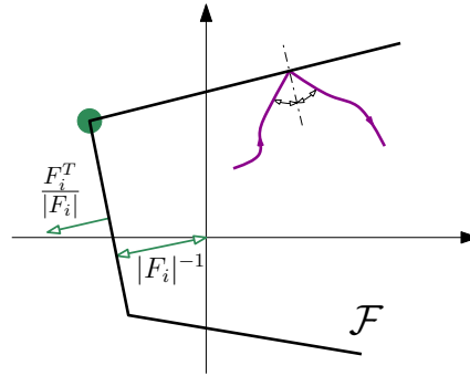
Figure 8.41: The polyhedral region \mathcal{F} for the case n = 2 with the representation of the effect of an impact.
