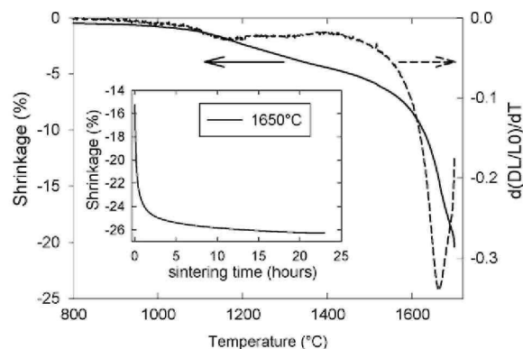
Fig. 5: Temperature dependence of the shrinkage and the shrinkage rate ( 10^\circ\text{C}/\text{min} heating rate). Inset: shrinkage vs. sintering time at 1650^\circ\text{C} (after heating to 1650^\circ\text{C} at 10^\circ\text{C}/\text{min} ).
