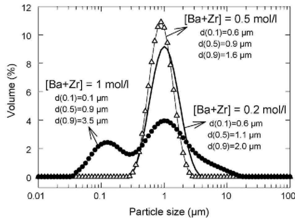
Fig. 4: Particle size distribution of powders precipitated from solutions with Ba + Zr concentration of 0.2 mol/l, 0.5 mol/l and 1 mol/l. (Other synthesis parameters: [\text{NaOH}] = 20 \text{ mol/l} , reaction time = 15 min).
