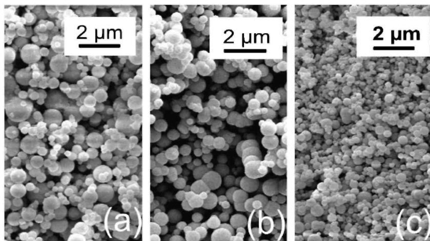
Fig. 3: Electron micrographs of powders precipitated from solutions with Ba + Zr concentration of (a) 0.2 mol/l, (b) 0.5 mol/l and (c) 1 mol/l. (Other synthesis parameters: [\text{NaOH}] = 20 \text{ mol/l} , reaction time = 15 min).
