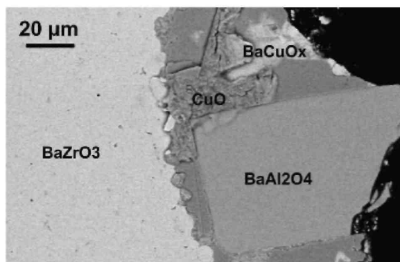
Fig. 7: Back-scattered electron micrograph of a polished cross-section through a \text{BaZrO}_3 rod sintered at 1650 °C for 13 h and immersed in a molten \text{BaO-CuO} flux at 1000 °C for 5 days.
