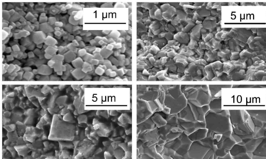
Fig. 6: Electron micrographs of fractures in samples sintered (a) at 1500^\circ\text{C} for 2 h, (b) at 1500^\circ\text{C} for 13 h, (c) at 1500^\circ\text{C} for 24 h and (d) at 1650^\circ\text{C} for 13 h.
