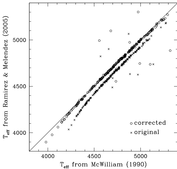
Fig. 8. Comparison between the Ramirez & Melendez (2005) and McWilliam (1990) T_{\text{eff}}/(V-K) relations in their original form (crosses), and after the correction proposed in the text (open circles).
