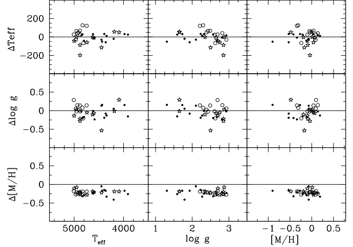
Fig. 6. Differences between atmospheric parameters obtained with our \chi^2 technique and literature values. Full circles are objects from Hekker & Melendez (1997), empty circles from Soubiran (2005), and stars from Takeda et al. (2008). Input data from Table 4.
