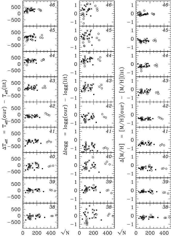
Fig. 5. \Delta T_{\text{eff}} , \Delta \log g , and \Delta [M/H] versus S/N for the nine Echelle orders. The plotted values are the differences with respect to the mean. Full circles are objects from Hekker & Melendez (2007), empty circles from Soubiran et al. (2005), and stars from Takeda et al. (2008).
