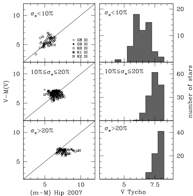
Fig. 10. Left columns present, for three different bins in the error of parallaxes and for all our program red clump stars, a comparison between the distance modulus obtained with the photometric parallaxes from Keenan & Barnbaum (2000) calibrations and distance modulus obtained with the revised Hipparcos parallaxes of van Leeuwen (2008). The lines represent the 1:1 correspondence. Each different spectral type is represented with a different symbol. The right columns give the corresponding distribution in V_T magnitudes.
