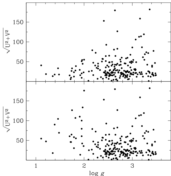
Fig. 11. Relation between orbital energy and surface gravity. The top panel is built assuming that all stars share the same luminosity class III, the bottom one assuming a luminosity class II for stars with \log g \leq 2 .
