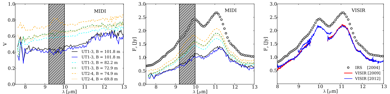
Fig. 2. VLTI/MIDI visibilities and correlated fluxes for HD 113766 A (left and middle panels, respectively). The baselines used and their lengths are reported in the caption of the left panel. Right panel shows the VISIR N -band spectrum at different epochs (2009 and 2012, in thick red and thin blue, respectively). The Spitzer /IRS spectrum is shown in open black circles in the middle and right panels.
