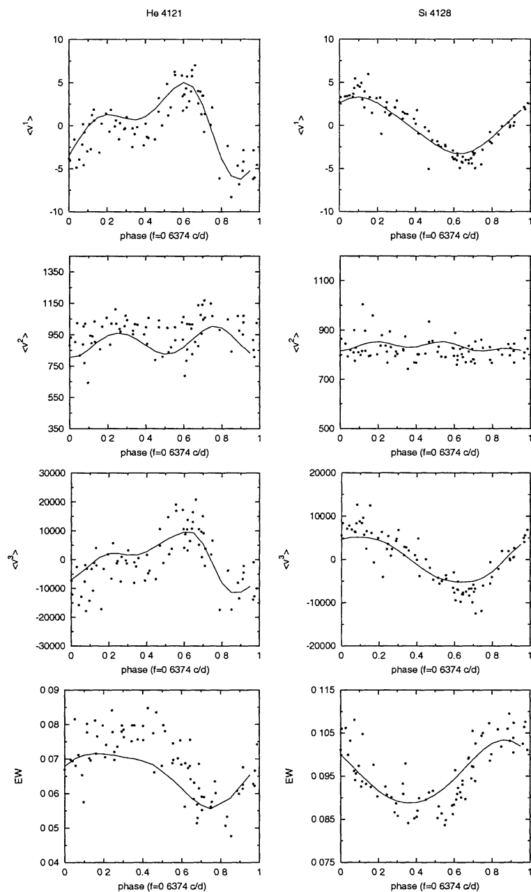
Figure 1. Phase diagrams of the first three moments (expressed in \text{km s}^{-1} , (\text{km s}^{-1})^2 and (\text{km s}^{-1})^3 respectively) and of the equivalent width (expressed in \text{\AA} ) for both the He 4121 \text{\AA} line (left) and the Si 4128 \text{\AA} line (right) for HD 131120. We show the observed values (dots) and those corresponding to the best spot model (solid line).
