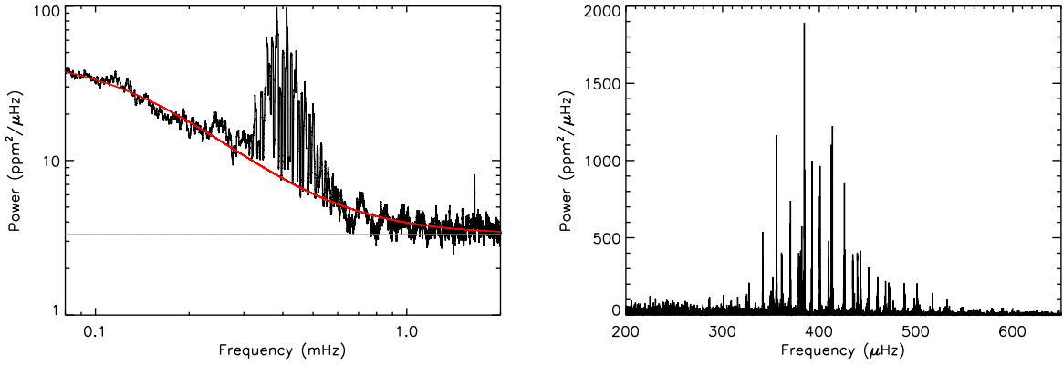
Fig. 2.— Power density spectrum of KIC7341231 computed with one year of Kepler observations. Left: Spectrum smoothed over a 2\text{-}\mu\text{Hz} boxcar. The red curve corresponds to a fit of a function of the type B(\nu) (see text) to the spectrum. The contribution from the photon noise is overplotted in gray. Right: Power density spectrum over the frequency range where oscillation modes are observed.
