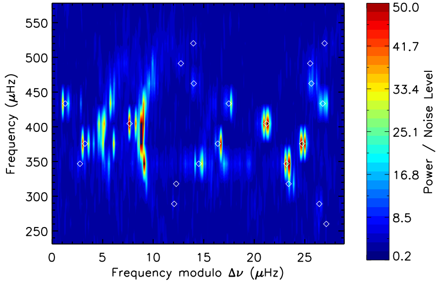
Fig. 3.— Échelle diagram of KIC7341231 folded with a large separation of \Delta\nu = 29\text{ }\mu\text{Hz} . For more clarity, the power spectrum was binned over a 0.2\text{-}\mu\text{Hz} boxcar and clipped at a maximum of 50 times the noise level. The white diamonds correspond to the mode frequencies predicted by the method of Benomar et al. (2012) (see text).
