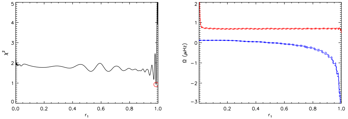
Fig. 13.— Left: Variations in the reduced \chi^2 value as a function of the radius r_1 . The red circle indicates the minimum of the function. Right: Optimal values of the core rotation \Omega_1 (red) and the surface rotation \Omega_2 (blue) as a function of r_1 . The dashed lines indicate the error bars.
