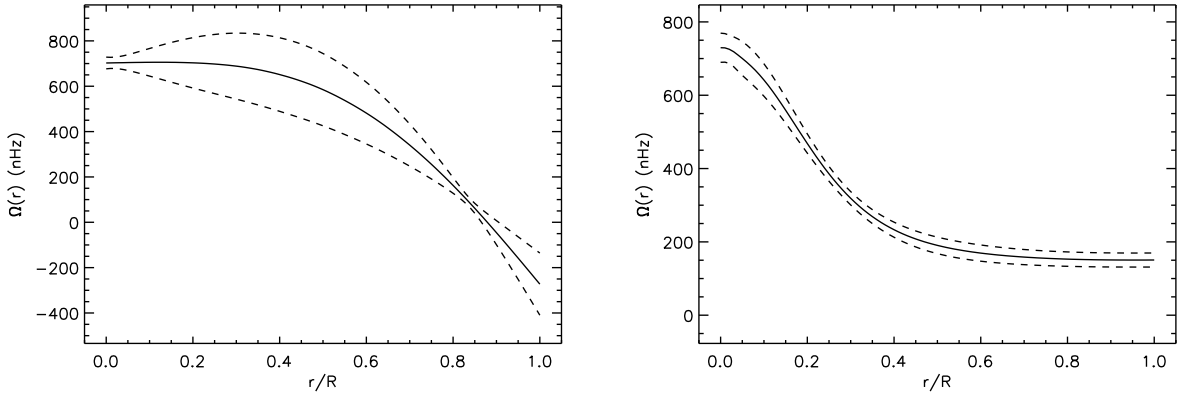
Fig. 15.— Left: Inverted rotation profile obtained with the RLS method (100 points, regularization with the second derivative and \mu = 100 ). The dashed lines indicate 1- \sigma error-bars. We note that apart from in the core, the averaging kernels are ill-localized and the inverted rotation rates are not reliable (see text). Right: Same as left panel using the OLA method.
