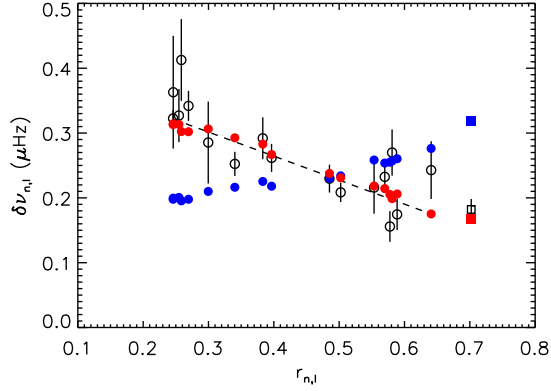
Fig. 10.— Rotational splittings of the modes as a function of the weighted radii r_{n,l} given by Eq. 6. The empty symbols ( l = 1 : circles, l = 2 : squares) correspond to the observations with 1- \sigma error bars, the filled blue symbols to an optimal solid-body rotation model and the filled red symbols to an optimal two-zone model.
