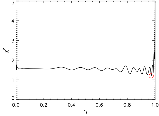
Fig. 14.— Same as the left panel of Fig. 13, but for a simulation (see text).
