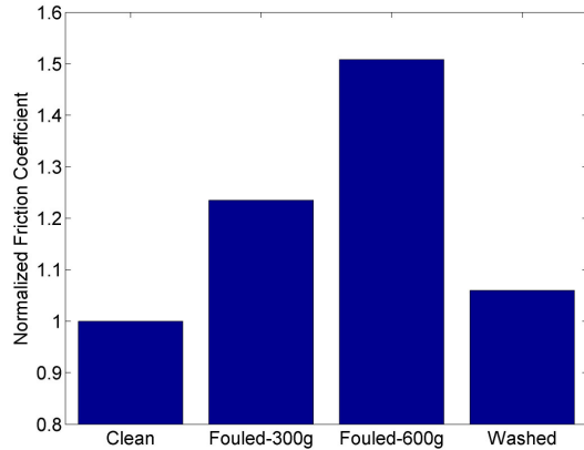
Figure 9: Normalized friction coefficients for dry operation
