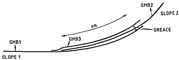
Fig. 3 Junction (in fan) at the cell corner between the slopes geomembranes
