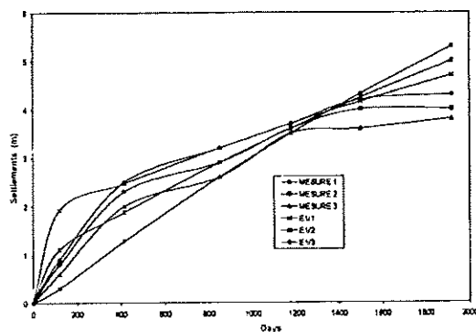
Figure 9. Comparison between on site and Gibson & Lo model
