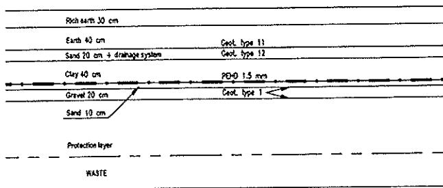
Figure 2. Waterproofing-drainage system for waste landfill capping
