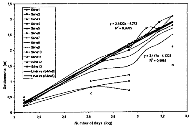
Figure 6. Linear regression on settlements versus time
