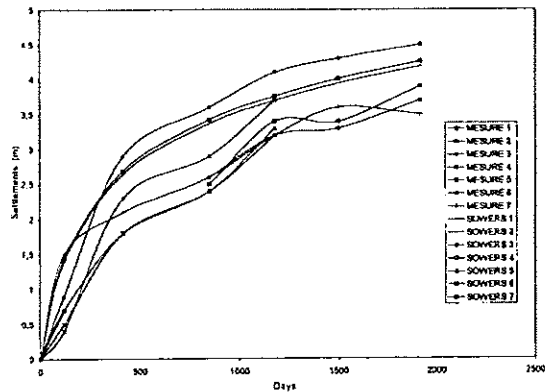
Figure 7. Comparison between on site measurements and Sowers model - ref. G1 [10]
