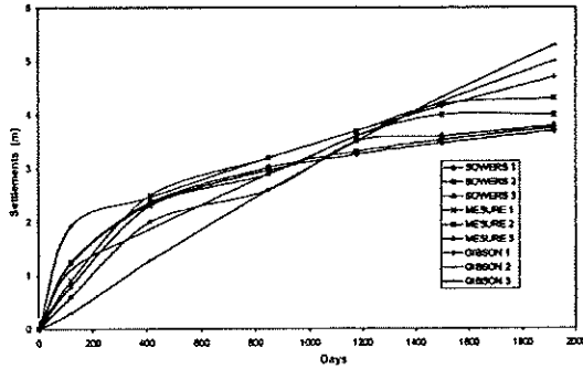
Figure 10. Comparison of models of Sowers and Gibson & Lo - Ref. D1
