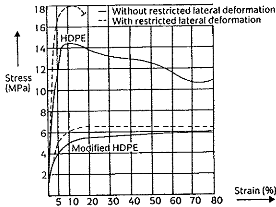
Figure 4. Stress-strain curves with or without lateral deformations [2]
