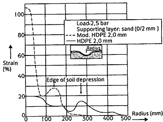
Figure 5. Deformations in the geomembrane during settlement test [2]
