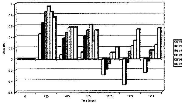
Figure 8. Gaps between Sowers model and on site measurements - Ref. E1 - measurements 1 to 7 [10]
