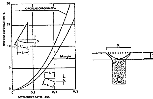
Figure 3. Deformation of the geomembranes versus settlement amplitude [1]
