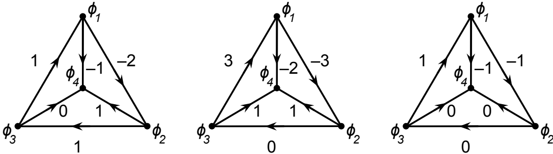
Figure 2: Coefficients p and q as labels of triangles representing bilinears in 4HDM
