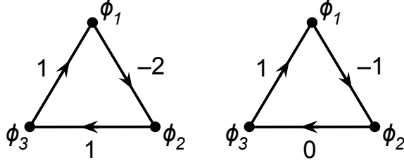
Figure 1: Coefficients p and q as labels of triangles representing bilinears in 3HDM
