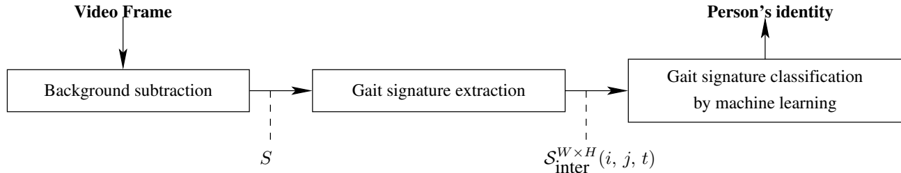
Fig. 3. Architecture of the gait recognition algorithm.
