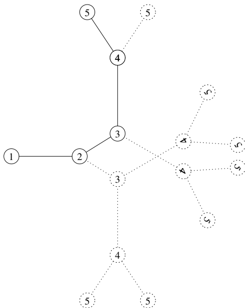
Figure 1: All 8 possible embeddings of a 5 vertex instance. The embedding described by the bit-string 000 is depicted with solid lines.
