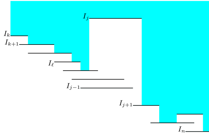
Figure 3: Recurrence relation of \mathcal{C}_k . If I_j is the first E -interval after I_k , then the cost divides into the cost of the intervals between k and j , plus \mathcal{C}_j
