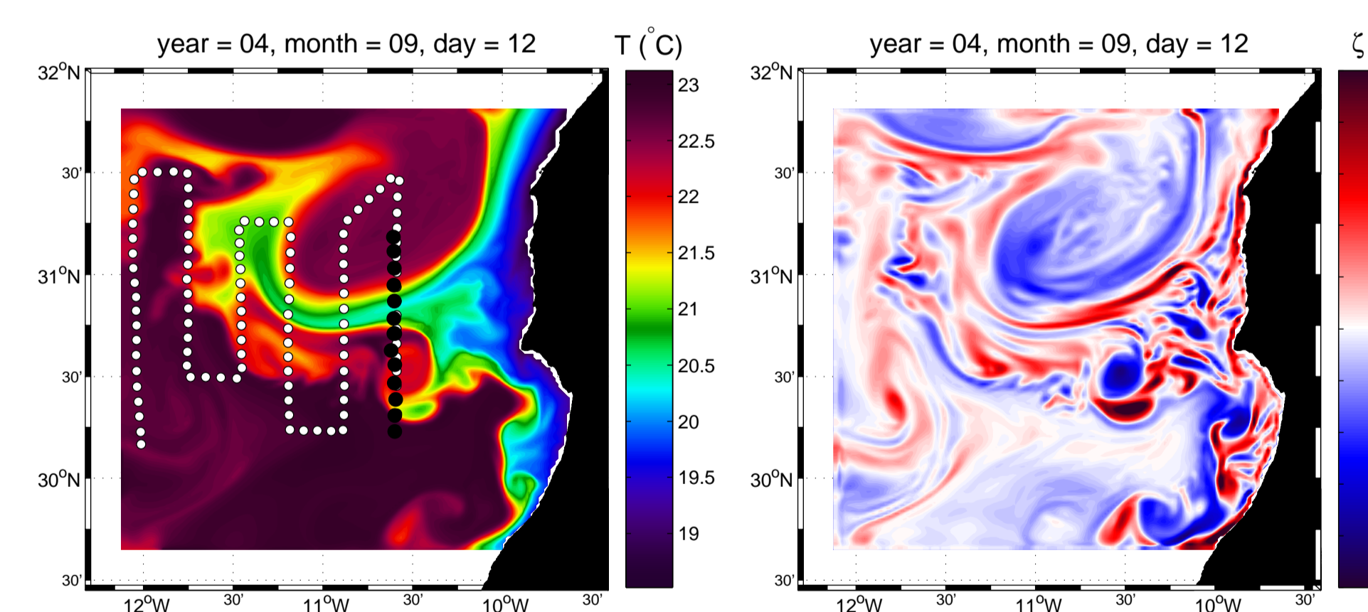
FIGURE 2: Modeled temperature and normalized relative vorticity at 10 m on September 12th. The SeaSoar tracks (white dots) and CTD transect (black dots) carried out during the cruise are superimposed on the temperature field.
