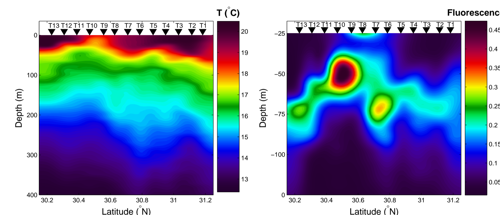
FIGURE 4: Analyzed fields of temperature and fluorescence with the data from the CTD section.
