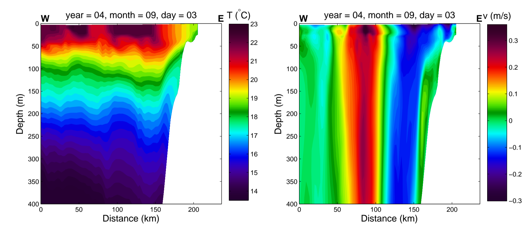
FIGURE 8: Transect at 31°N for modeled temperature and meridional velocity on September 3rd.
