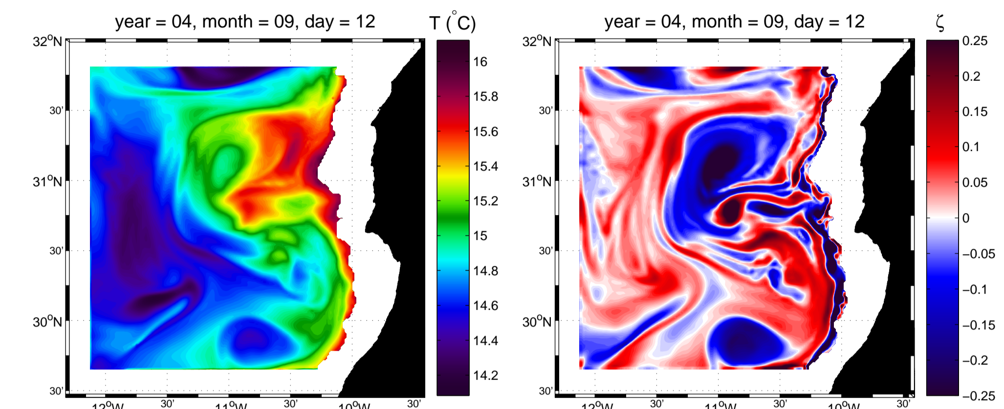
FIGURE 7: Temperature and normalized relative vorticity fields at 300 m on September 12th.
