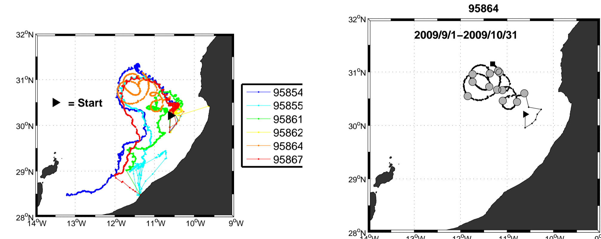
FIGURE 5: Trajectories of the drifters (left) launched on September 3rd, 2009. Drifter n° (right) 95864 has its drogue at 300 m.
