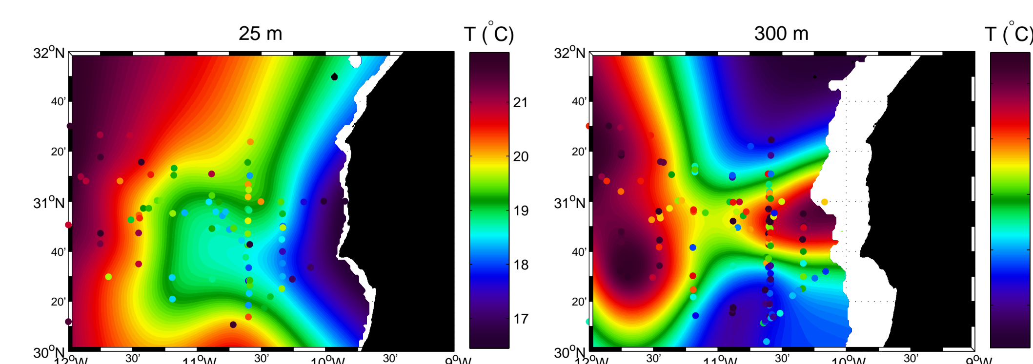
FIGURE 6: Temperature field at 25 and 300 m, constructed using all the measurements made during the cruise.
