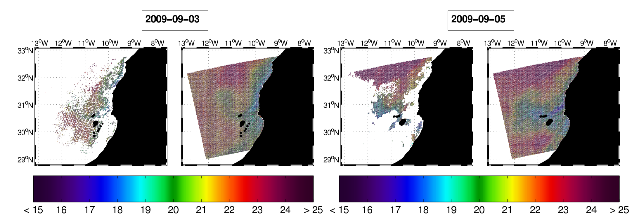
FIGURE 9: Drifter positions and reconstruction of SST field for September 3rd and 5th, 2009.
