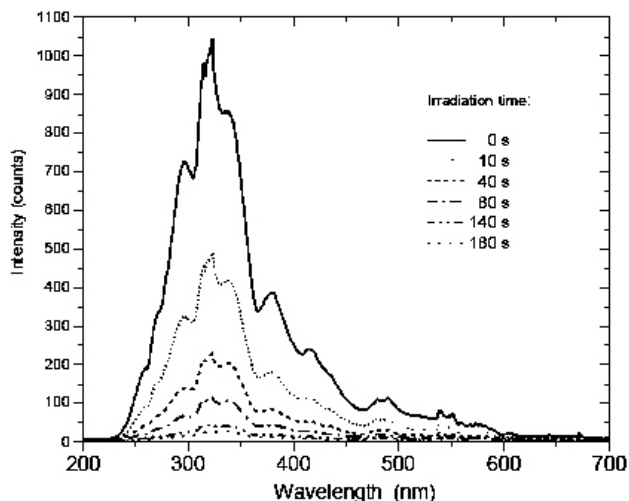
FIGURE 5. IL spectra for green Fluorite as a function of the irradiation time from 0 to 180 s. Proton beam current on the sample was 150 nA.
