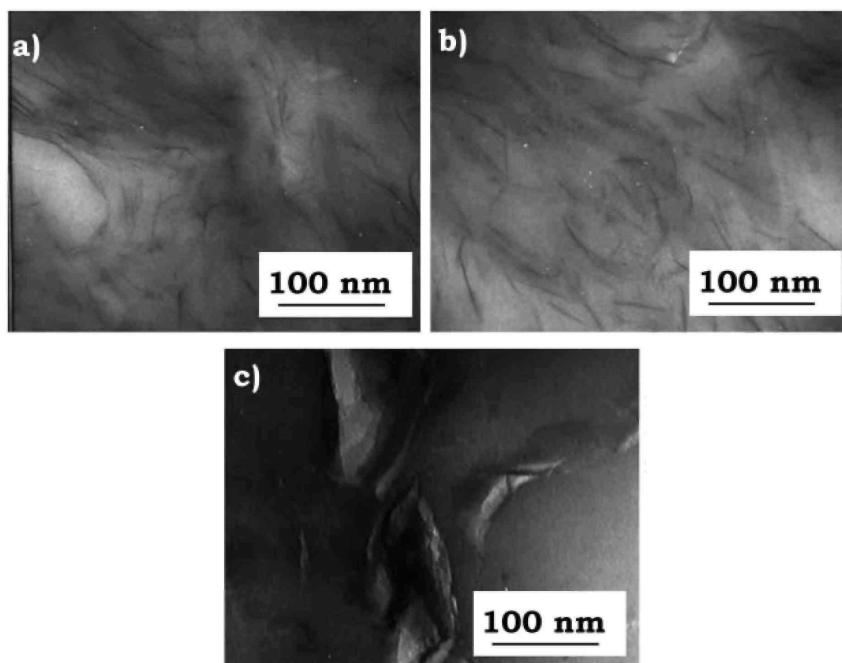
Fig. 2 TEM images for the PCL/MMT-(CH 2 CH 2 OH) x nanocomposites prepared in the presence of Sn(Oct) 2 : a) x = 100%, b) x = 50%, c) x = 0 % (see Table 3).
