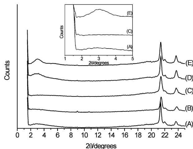
Fig. 1 XRD patterns for PCL/MMT-(CH 2 CH 2 OH) x nanocomposites prepared in the presence of Sn(Oct) 2 . Effect of the content of monohydroxylated ammonium cations used in the Na exchange of native MMT: (A) x = 100\% , (B) x = 75\% , (C) x = 50\% , (D) x = 25\% , (E) x = 0\% . The insert shows a zoom of the low angle area (1 to 5°) for curves (A), (C) and (E).
