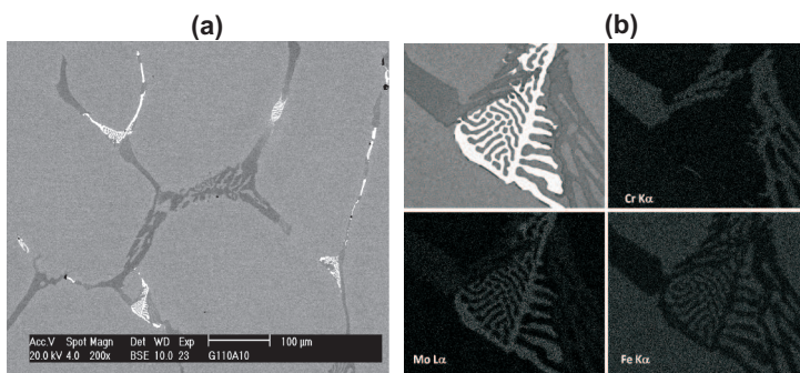
Figure 6.a: Eutectic carbides network on cr-steel after dta test – fishbone-like m_7c_3 (grey) and fine-lamellar m_6c (light) nitral etching
