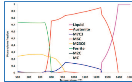
Figure 4.a: Phase volume fraction evolution on cr-steel - equilibrium conditions
