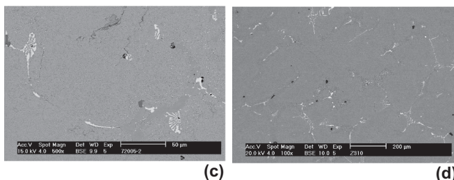
Figure 7.c: Semi-hss 2 (close to the scrap diameter) – network of eutectic m_7c_3 (bulk, grey) and m_6c (light) at grain boundaries, in a tempered Martensitic matrix. Nitral etching.
