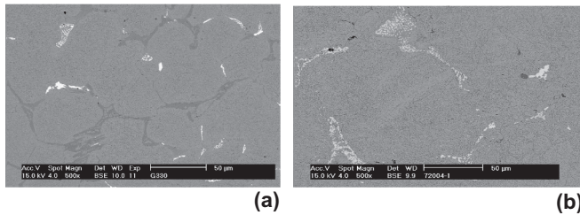
Figure 7.a: CR- steel (near the surface of the shell) network of eutectic m_7c_3 (fishbone-like, grey) and m_6c (light) carbides at grain boundaries, in an untempered Martensitic matrix. Nitral etching.
