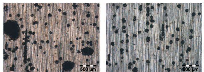
Figure 9: Overview of corrosion pits on cr steel (left) and semi-hss 3 (right) surfaces
