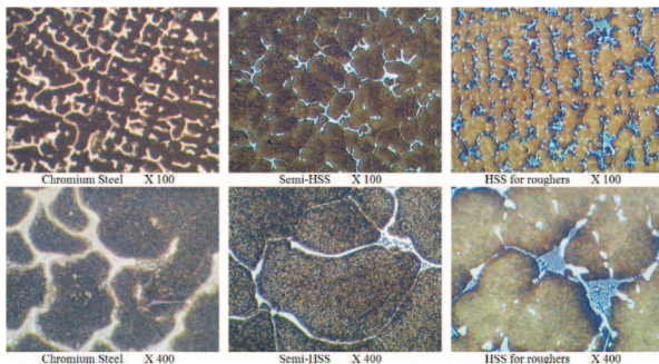
Figure 3: Overview of work rolls microstructures for roughing stands – 400x nital etching
