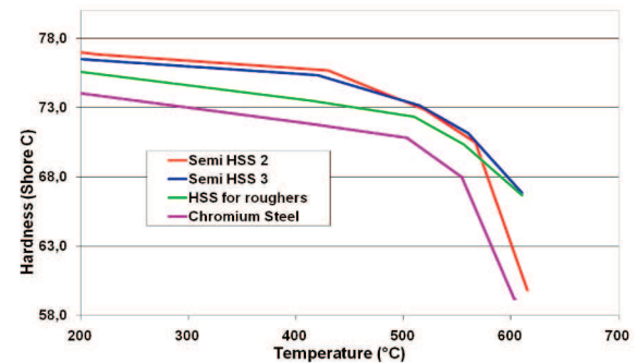
Figure 8: Hot hardness (shore c) on semi-hss grades 2 and 3, cr-steel, and hss for roughers (as reference)
