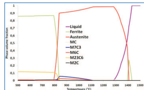
Figure 4.d: Phase volume fraction evolution on semi-hss 3 - equilibrium conditions
