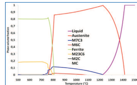
Figure 4.c: Phase volume fractions on semi-hss 2 - equilibrium conditions
