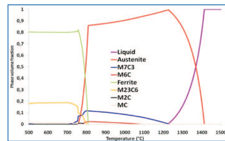
Figure 4.b: Phase volume fractions on semi-hss 1 - equilibrium conditions
