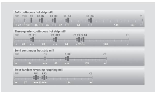
Figure 10: Layouts of hot strip roughing mills
