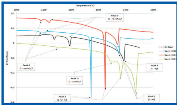
Figure 5: Solidification sequences on the four studied alloys during dta cooling stage at 5°C/min
