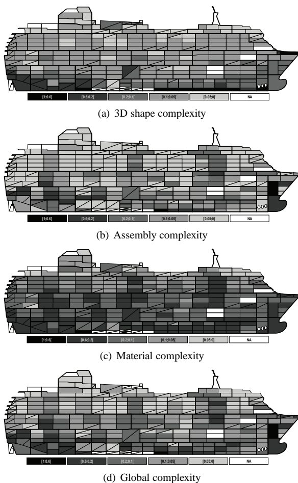
Figure 4: Complexity of a cruise ship
