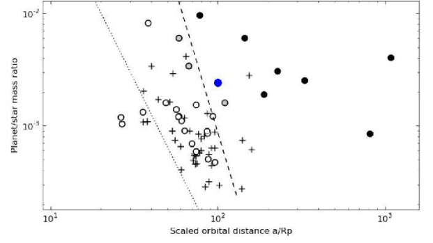
Fig. 13: Corot-23b (blue dot) added on the M_{pl}/M_* vs a/R_p diagram proposed by Pont et al. (2011). Corot-23b appears to lie outside the band of circularized planets.
