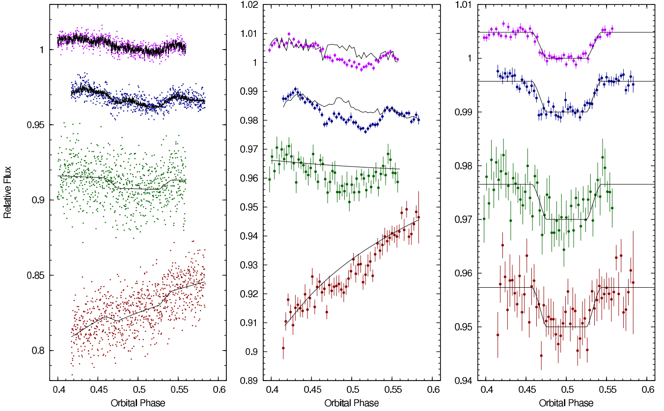
Figure 1. In each of the above three plots, from top to bottom, the data were taken at 3.6, 4.5, 5.8 and 8.0 \mu\text{m} . Relative flux offsets were applied to datasets for clarity. Left: Raw Spitzer data with the best-fitting trend and occultation models superimposed. Middle: The same data binned in phase ( \Delta\phi = 0.003 \sim 3.4 min) with the best-fitting trend models superimposed. Right: The binned data after dividing by the best-fitting trend models, and with the best-fitting occultation models superimposed. The error bar on each binned measurement in the panels in the middle and on the right is the standard deviation of the points within the bin.
