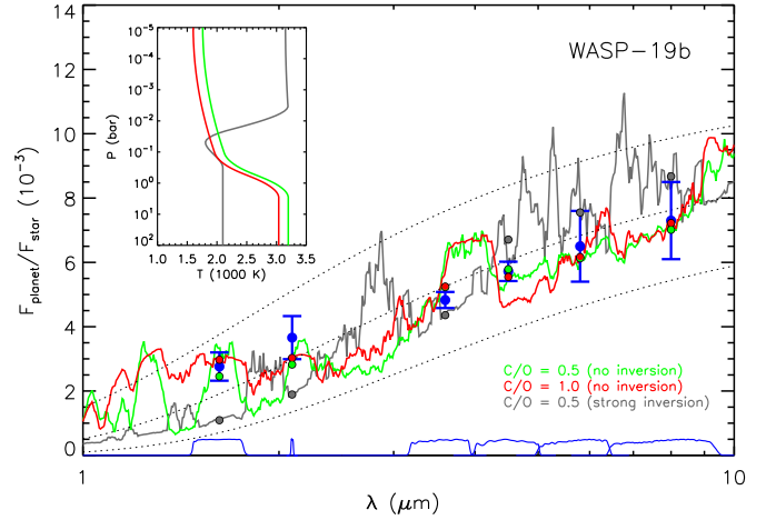
Figure 4. Spectral energy distribution of WASP-19b relative to that of its host star. The blue dots are our fitted planet-to-star flux density ratios. The observation-band transmission curves are shown along the abscissa. The planet-to-star flux density ratios indicate the absence of a strong temperature inversion. Two model-atmosphere spectra are shown, each of which fits the data and lacks a temperature inversion. One model has a C/O ratio of 0.5 and is shown as a green line. The other has a C/O ratio of 1.0 is depicted by a red line. The corresponding band-integrated model fluxes are shown as dots with the same colour scheme. The models' pressure–temperature profiles down to 100 bar are shown in the inset. Assuming zero albedo, the maximum dayside-to-nightside redistribution efficiency is 20 per cent for the C-rich model and 34 per cent for the O-rich model. The three dotted lines show planetary black bodies with temperatures of 1800, 2250 and 2900 K (chosen to give a sense of scale to the spectra) divided by a stellar spectrum.
