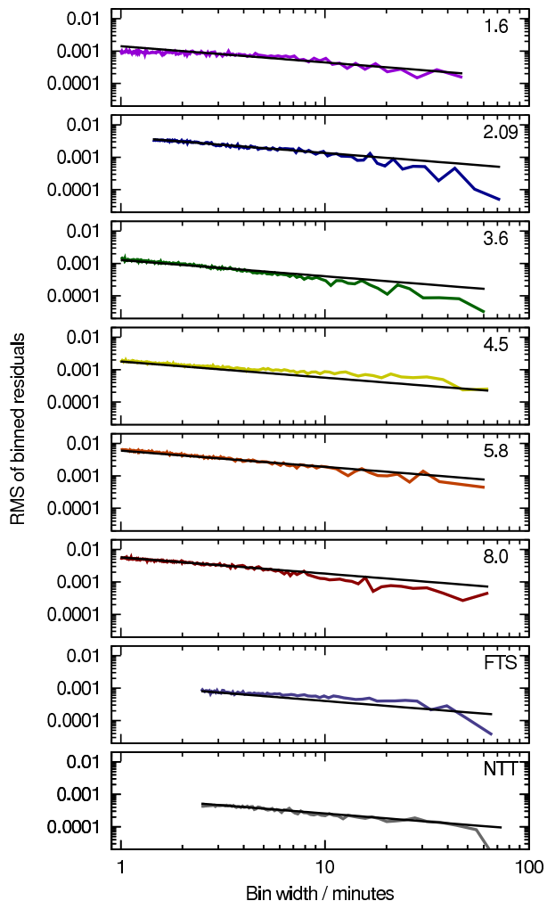
Figure 2. RMS of the binned residuals for, from top to bottom, the pre-existing HAWK-I occultation photometry at 1.6 \mu\text{m} and 2.1 \mu\text{m} , the new Spitzer occultation photometry at 3.6, 4.5, 5.8 and 8.0 \mu\text{m} , and the pre-existing FTS and NTT transit photometry. The solid black lines, which are the rms of the unbinned data scaled by the square root of the number of points in each bin, show the white-noise expectation. The ranges of bin widths are appropriate for the datasets' cadences and durations.
