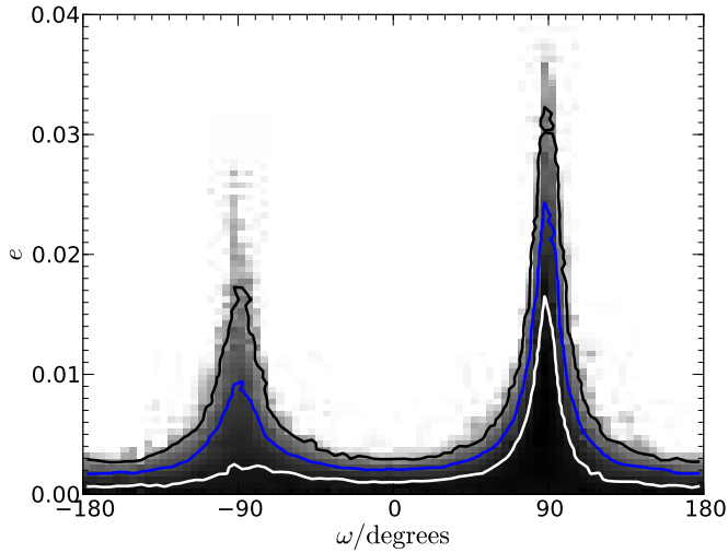
Figure 5. The MCMC posterior distributions of e and \omega . The white, blue and black contours are, respectively, the 1-, 2- and 3- \sigma confidence limits. The shading of each bin is proportional to the logarithm of the number of MCMC steps within. The available data exclude large values of e for any orbital orientation, and only very small values of e are permitted unless |\omega| \approx 90 .
