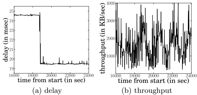
Figure 1: Details of the times series for PPMs measured between Cambridge and Köln
