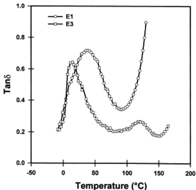
Fig. 4. Temperature dependence of \tan \delta for the E1 and E3 samples of the MEM series (Table 1).
