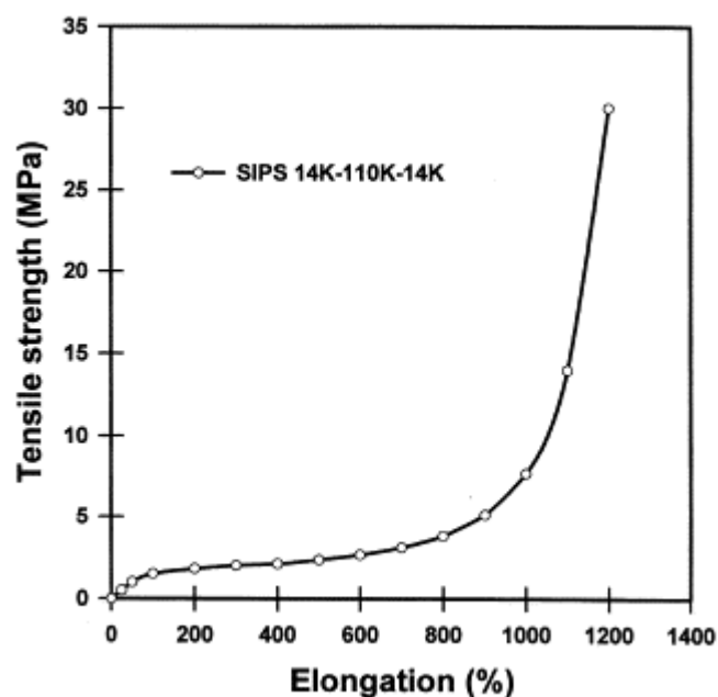
Fig. 7. Tensile curve for the SIPS triblock of 14,000–112,000–14,000.
