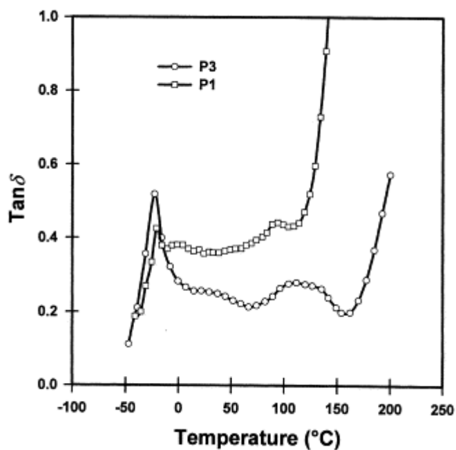
Fig. 3. Temperature dependence of \tan \delta for the P1 and P3 samples of the MnPM series (Table 1).
