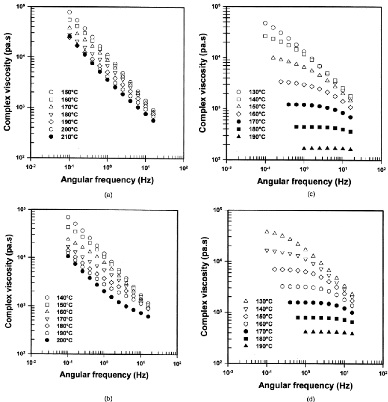
Fig. 9. Plots of complex viscosity vs. angular frequency at different temperatures for: (a) I1; (b) B1; (c) P1 and (d) E1 (Table 1).
