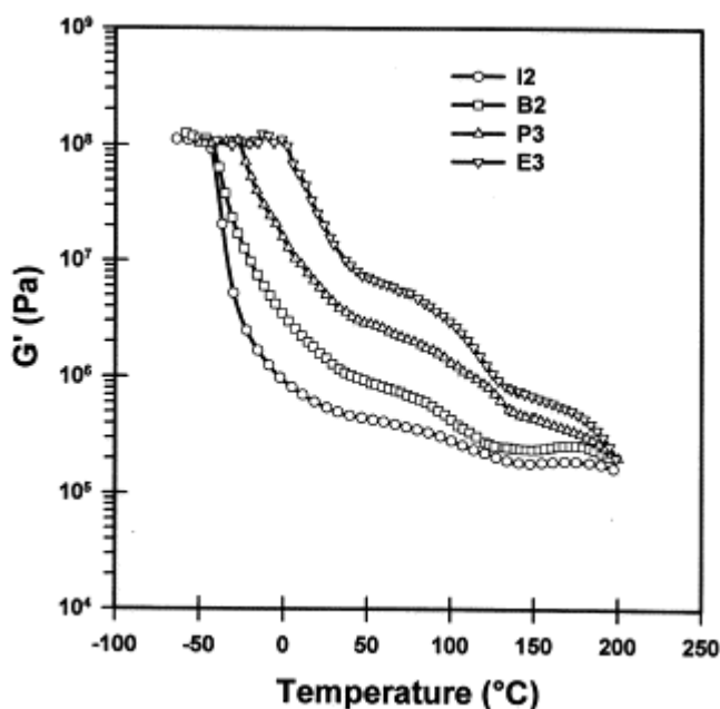
Fig. 5. Temperature dependence of storage modulus, G' , for the I2, B2, P3 and E3 samples (Table 1). The PMMA wt% is ca. 22–23% for each sample.
