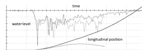
Figure 5. Results of two model tests with a self-propelled tug-barge combination leaving a lock: water level at the closed lock gate and longitudinal position of the vessel as a function of time. Source: Flanders Hydraulics Research.
