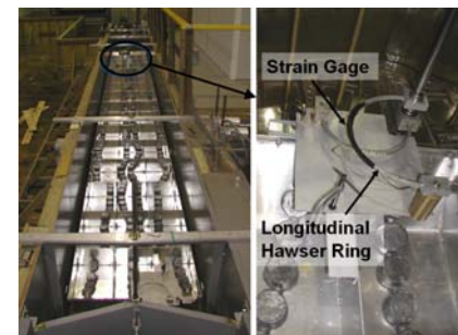
Fig 2: Hawser-pull (force link) devices
