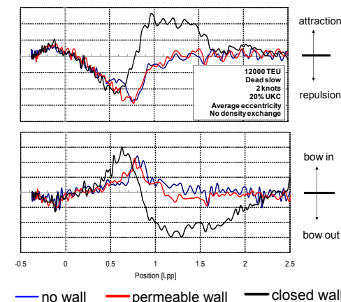
Figure 2. Lateral force (above) and yawing moment (below) on a self-propelled guided ship model during (eccentric) lock exit: effect of approach wall layout. Source: Flanders Hydraulics Research commissioned by Consorcio Pos Panamax on behalf of Panama Canal Authorities, [1], [2].
