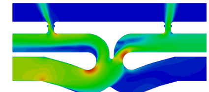
Figure 2 : CFD flow simulation in component of filling-emptying system (Courtesy: GUPC/CICP)
