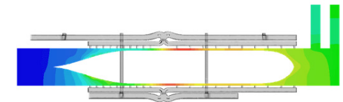
Figure 4 : CFD flow simulation around vessel in lock chamber (Courtesy: CPP)
