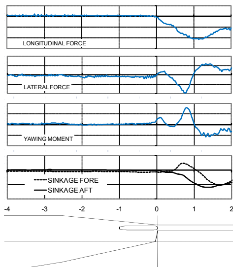
Figure 3. Captive model test with a bulk carrier entering the Pierre Vandamme Lock (Zeebrugge, Belgium) with asymmetric approach at constant speed. Longitudinal position convention: see Figure 1. Towing tank for maneuvers in shallow water (co-operation Flanders Hydraulics Research – Ghent University), Antwerp.
