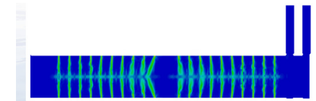
Figure 3 : CFD flow simulation in lock chamber (Courtesy: GUPC/CICP)
