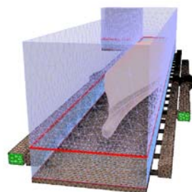
Figure 1: 3D model of the lock chamber, its F-E system and the design vessel
