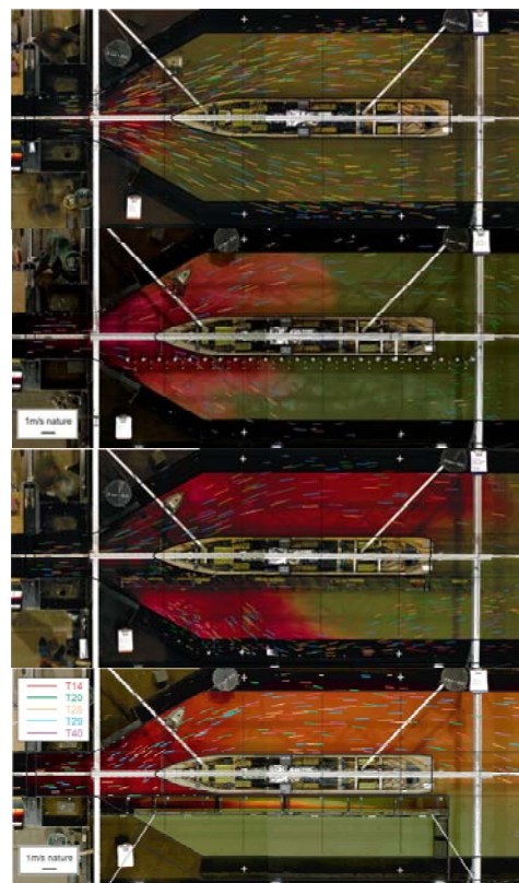
Figure 4. Effect of approach structure configuration on surface current pattern due to density exchange flow: no wall – ‘invisible’ wall (series of piles) – permeable wall – closed wall. Source: Flanders Hydraulics Research commissioned by Consorcio Pos Panamax on behalf of Panama Canal Authorities; [1], [2].
