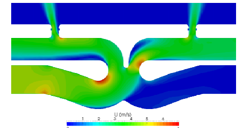
Figure 2: central flow connection
