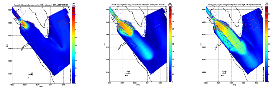
Figure 3: Illustration of draft-weighted average velocity (over 15.2 m) at different stages of the opening sequence.
