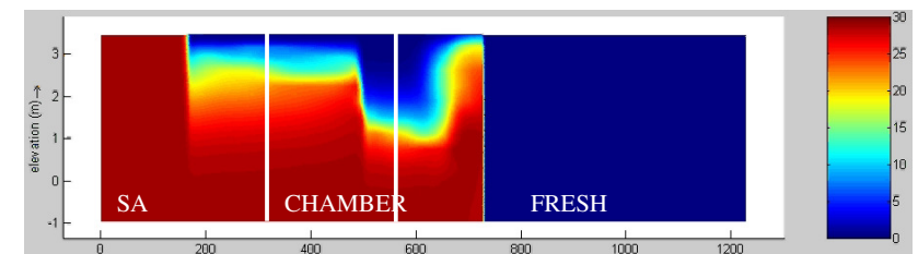
Figure 4: Modelled density flow in lock chamber for the Seine Scheldt West Canal
