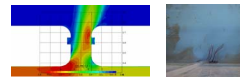
Figure 3: numerical calculation Vs observation on physical model
