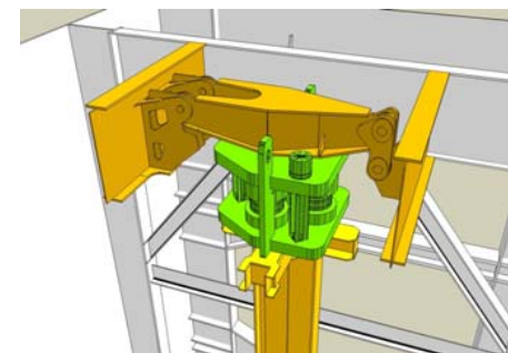
Fig. 5. Load limiting device arrangement at the top of the lower wagon column. Tekla 3-D model.
