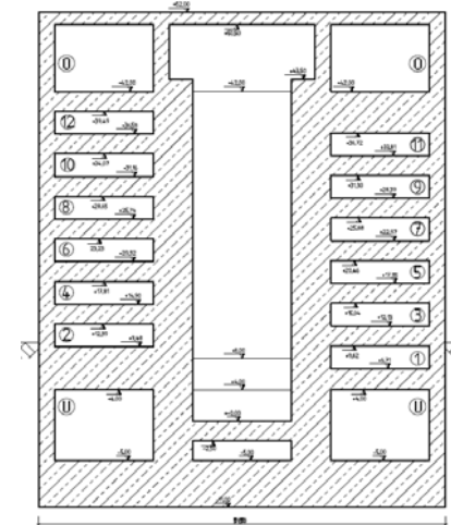
Figure 2: Cross-section of the lock with integrated water saving and exchange basins
