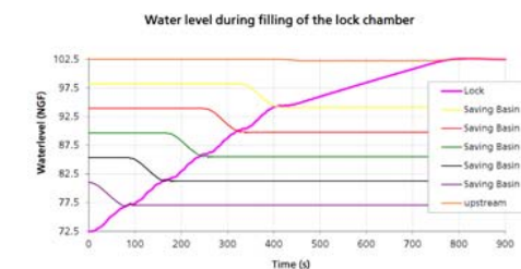
Fig 2: Levels during filling of lock
