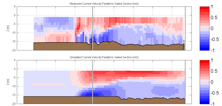
Figure 2: Typical calibration result: Longitudinal variation (at 300–1200m from upper gates) of a) measured velocity (10:45-10:53), b) modeled velocity (10:49).
