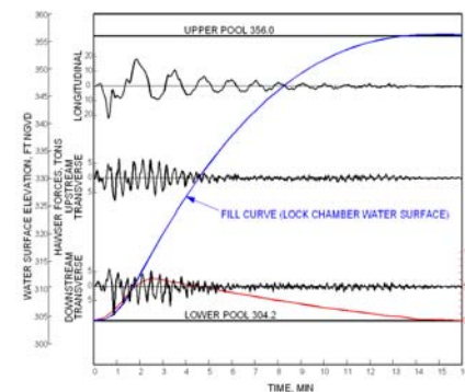
Fig 3: Physical model lock filling data
