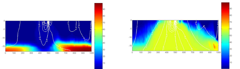
Figure 5: today's groundwater salinity through the existing canal (left); salinity 32 years after the introduction of the canal (right)
