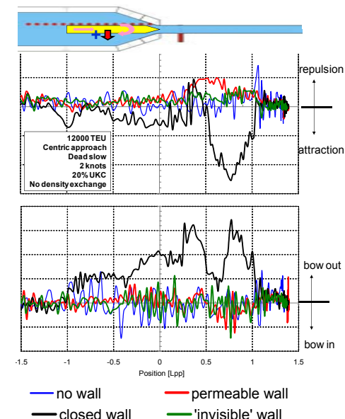
Figure 1. Lateral force (above) and yawing moment (below) on a self-propelled guided ship model during lock approach: effect of approach wall layout. Zero position is sketched above. Source: Flanders Hydraulics Research commissioned by Consorcio Pos Panamax on behalf of Panama Canal Authorities, [1], [2].
