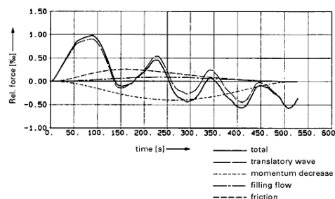
Fig 1: Forces on vessel during filling (RWS, 2000)
