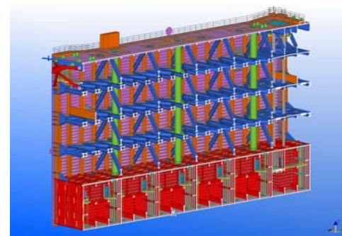
Fig. 4. Longitudinal section of a lock rolling gate showing buoyancy chambers, trusses and the upper support bracket. Tekla 3-D model.
