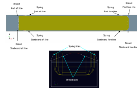
Figure 4: Mooring lines system configuration set in Adams software
