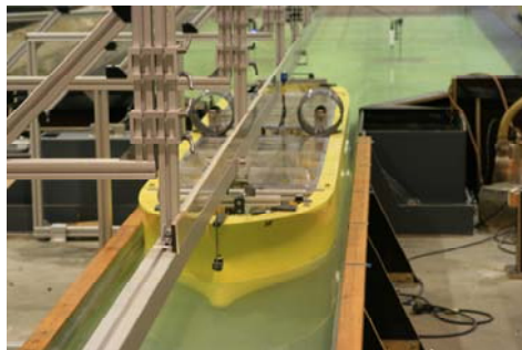
Figure 9. Lock entrance facility for self-propelled, laterally guided ship models at Flanders Hydraulics Research (photo Flanders Hydraulics Research)
