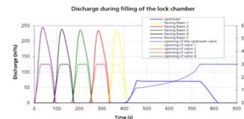
Fig 3: Discharges during filling of lock
