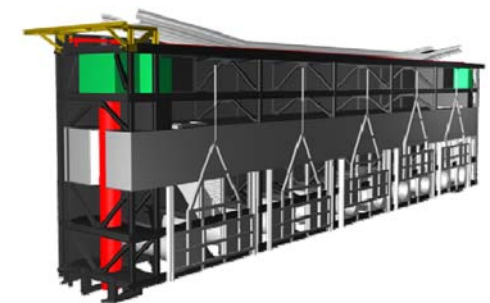
Fig. 3. Lay-out of Malamocco Lock gate in Venice, showing one hydro-foot tube in red.
