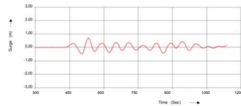
Fig 5: Vessel motions during filling of lock
