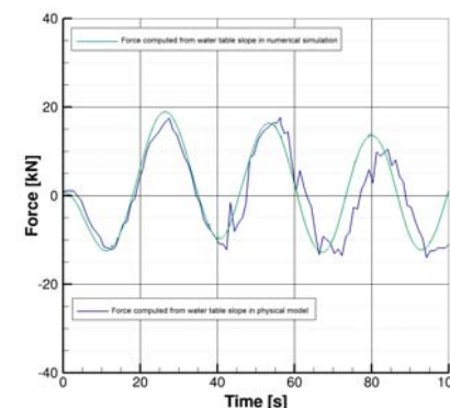
Figure 3: Ship forces computed from water table slope of physical and numerical model
