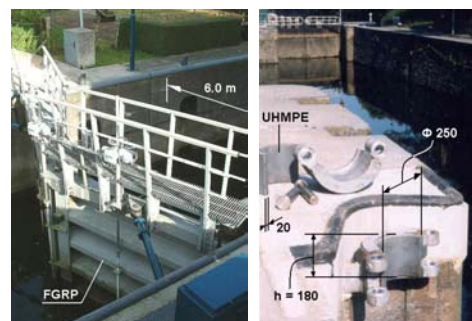
Fig. 1. FRP gate of the Spiering Lock, Werkendam (left) and UHMPE top hinge of the Tilburg Lock in Wilhelmina Canal (right)
