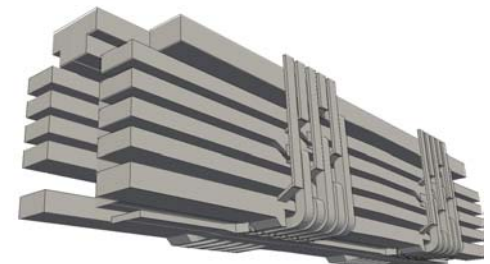
Figure 3: Hydraulically relevant surfaces of the lock
