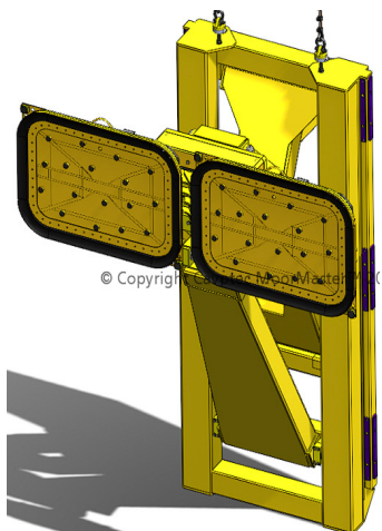
Figure 3 - Conceptual design of new prototype
