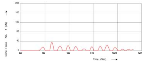
Fig 6: Mooring line force during filling of lock
