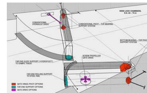
Fig. 4. Options of miter gates with far end supports for very wide lock chambers
