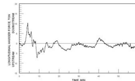
Fig 4: Hawser forces on a tow moored in the upper approach during lock filling
